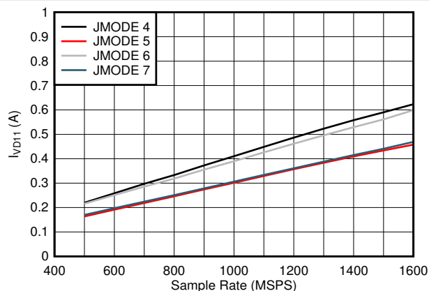
FIG 7-86. Quad Channel, I_{VD11} vs F_S and JMODE 4 - 7
