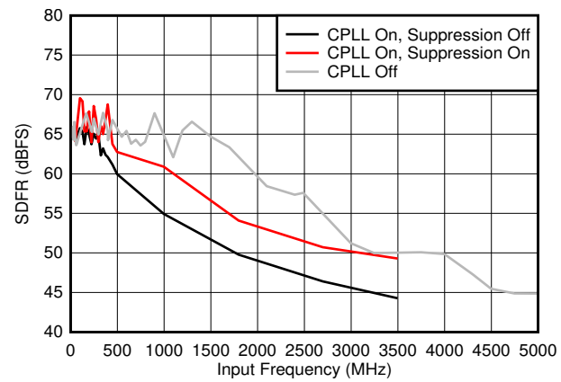
Figure 7-40. SFDR vs F_{IN} and C-PLL modes
