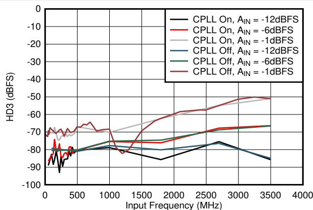
FIG 7-53. HD3 vs A_{IN} and C-PLL
