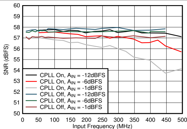
FIG 7-55. SNR vs A_{IN} and C-PLL
