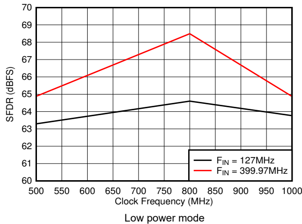
7-27. SFDR vs Sample Rate
