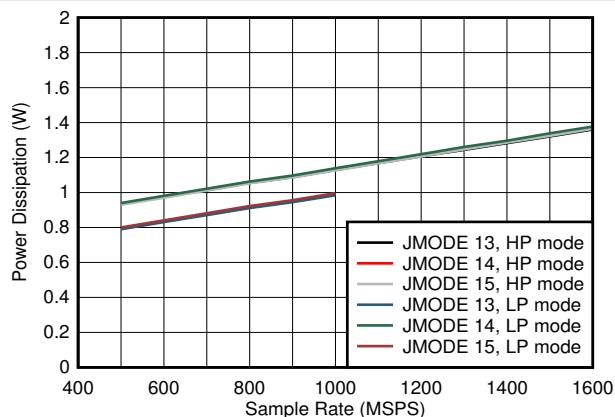
7-102. Single Channel, Power Dissipation vs F_S and JMODE 13 - 15
