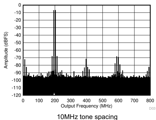
Figure 7-70. Two Tone FFT at 1798MHz
