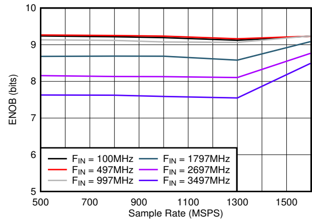
7-26. ENOB vs Sample Rate
