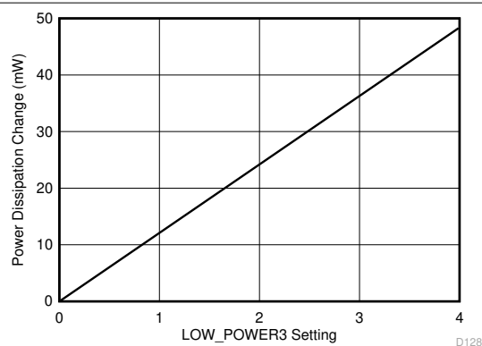
図 8-11. Power Dissipation Change vs LOW_POWER3 register setting
