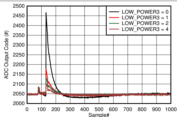
図 8-10. Background Calibration Core Transition In Low Power Mode
