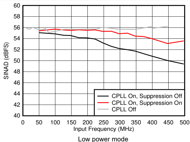
7-46. SINAD vs F_{IN} and C-PLL modes
