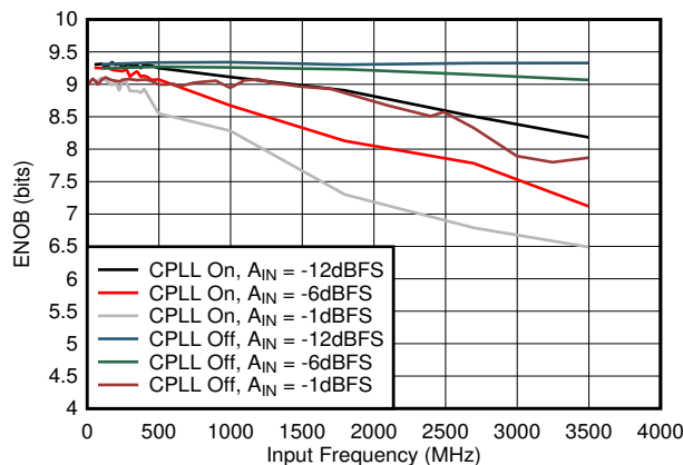
Figure 7-51. ENOB vs A_{IN} and C-PLL
