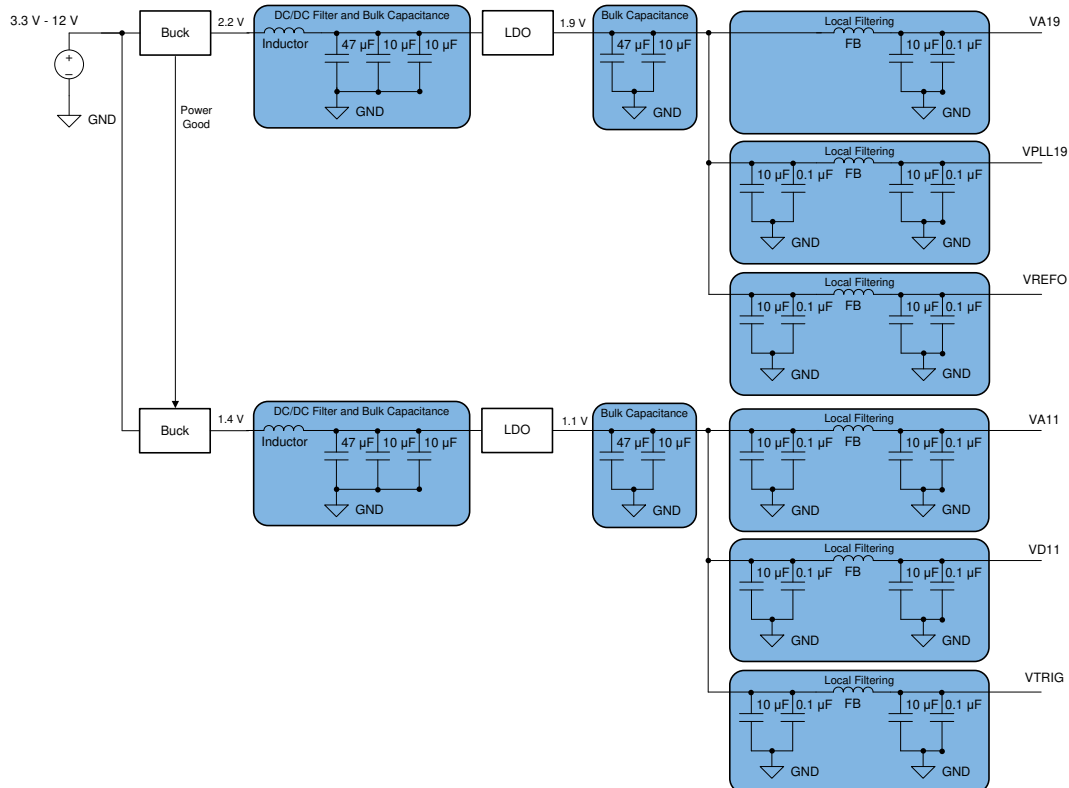
图 9-3. LDO Linear Regulator Approach Example
