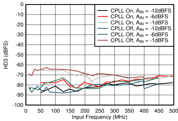
Figure 7-59. HD3 vs A_{IN} and C-PLL
