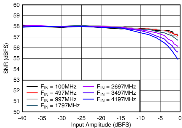
7-33. SNR vs A_{IN}
