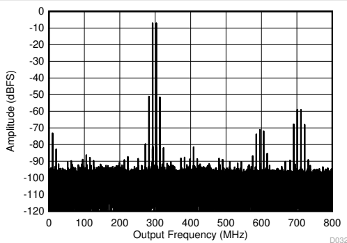
7-71. Two Tone FFT at 3498 MHz
