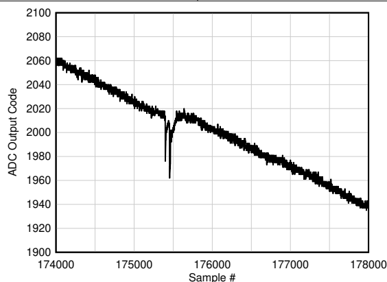
7-125. Background Calibration Core Transition (offset voltage)
