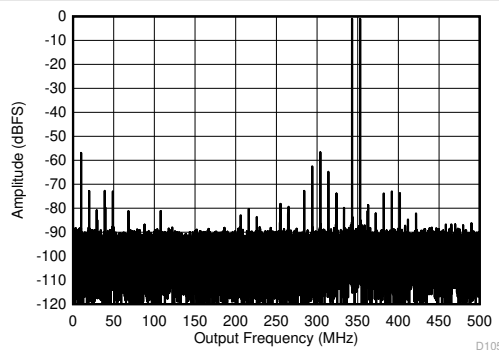
7-72. Two Tone FFT at 348 MHz
