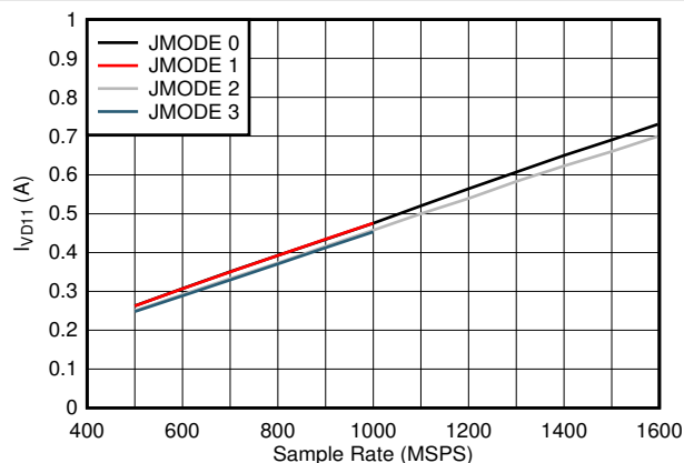
FIG 7-85. Quad Channel, I_{VD11} vs F_S and JMODE 0 - 3
