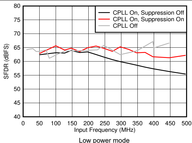
7-44. SFDR vs F_{IN} and C-PLL modes
