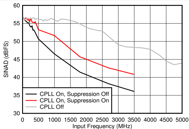
7-42. SINAD vs F_{IN} and C-PLL modes
