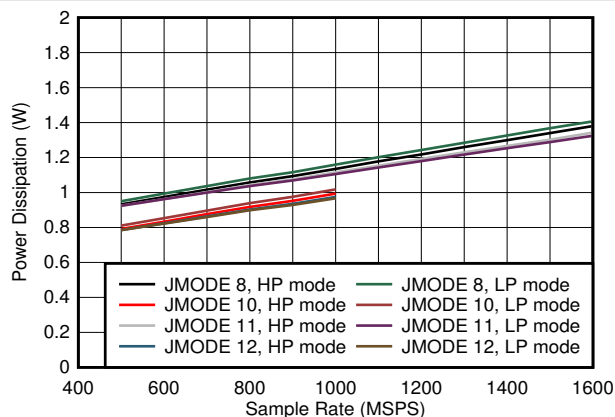
7-101. Single Channel, Power Dissipation vs F_S and JMODE 8 - 12
