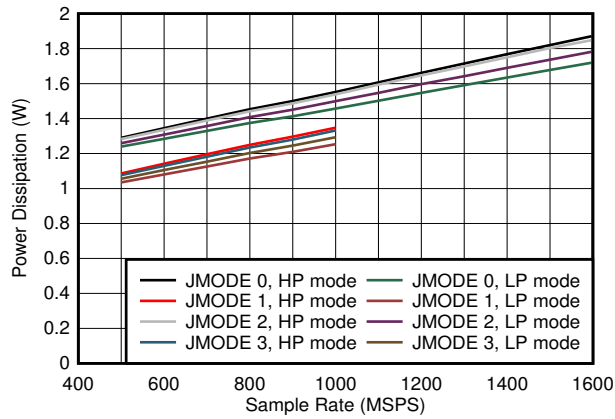
7-89. Dual Channel, Power Dissipation vs F_S and JMODE 0 - 3
