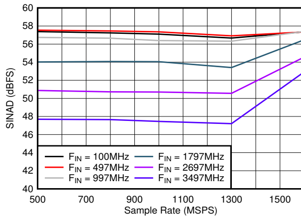
7-25. SINAD vs Sample Rate
