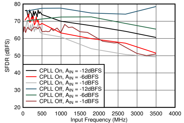
Figure 7-48. SFDR vs A_{IN} and C-PLL
