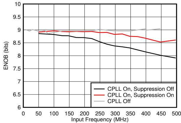
Figure 7-47. ENOB vs F_{IN} and C-PLL modes
