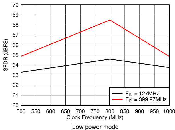
7-29. SFDR vs Sample Rate
