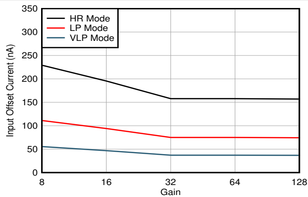
FIG 6-4. Input Offset Current vs Gain
