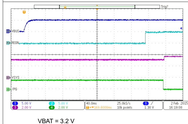
Figure 9-4. Power Up with Charge Disabled
