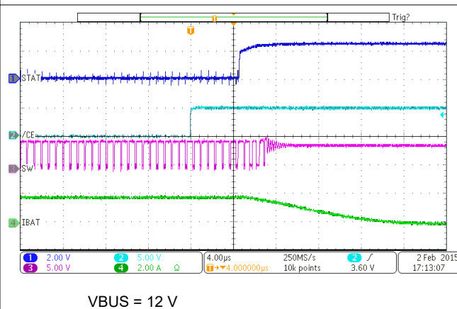
Figure 9-7. Charge Disable
