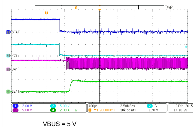
Figure 9-6. Charge Enable
