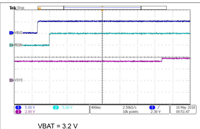
Figure 9-3. Power Up with Charge Disabled
