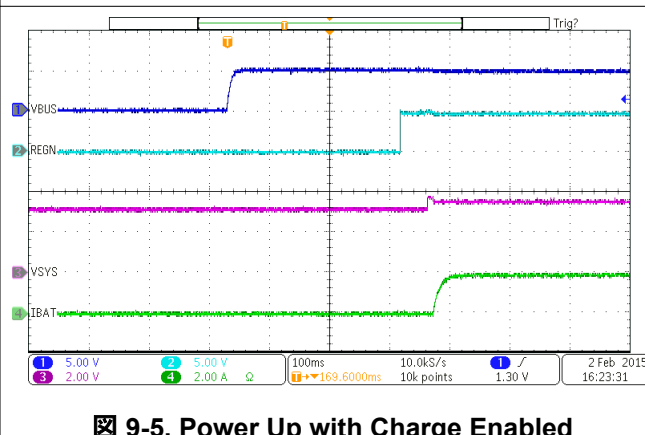
Figure 9-5. Power Up with Charge Enabled
