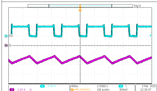
FIG 9-10. PWM Switching Waveform
