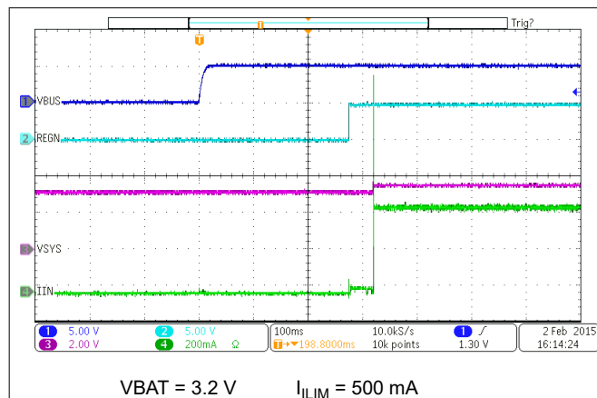
Figure 9-2. Power Up from USB100
