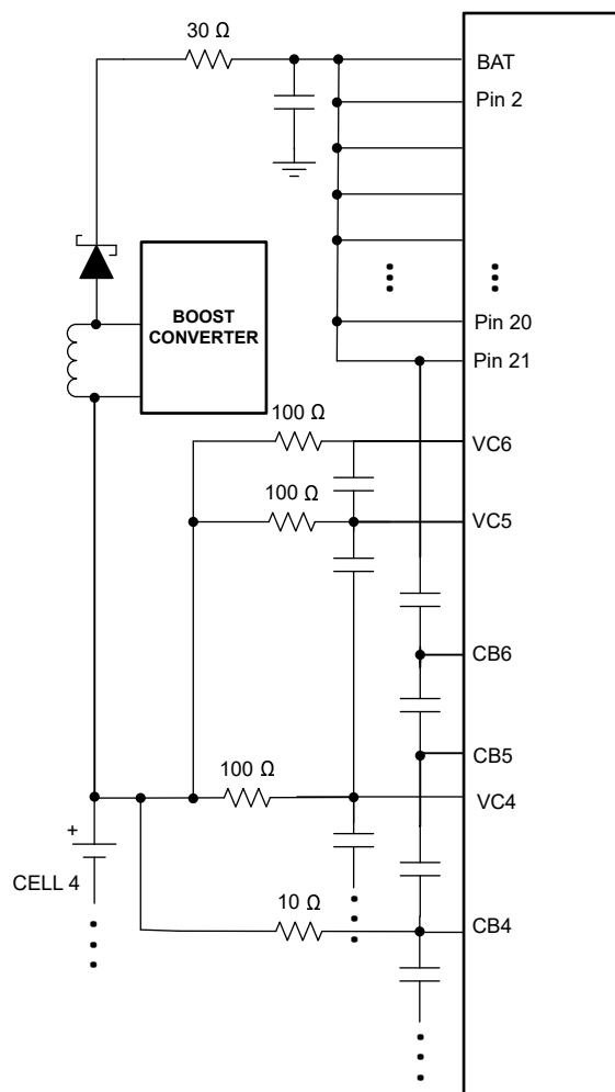
図 9-4. Unused VC and CB Channels - 4S
