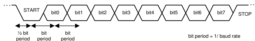
図 8-23. UART Communication to Host
