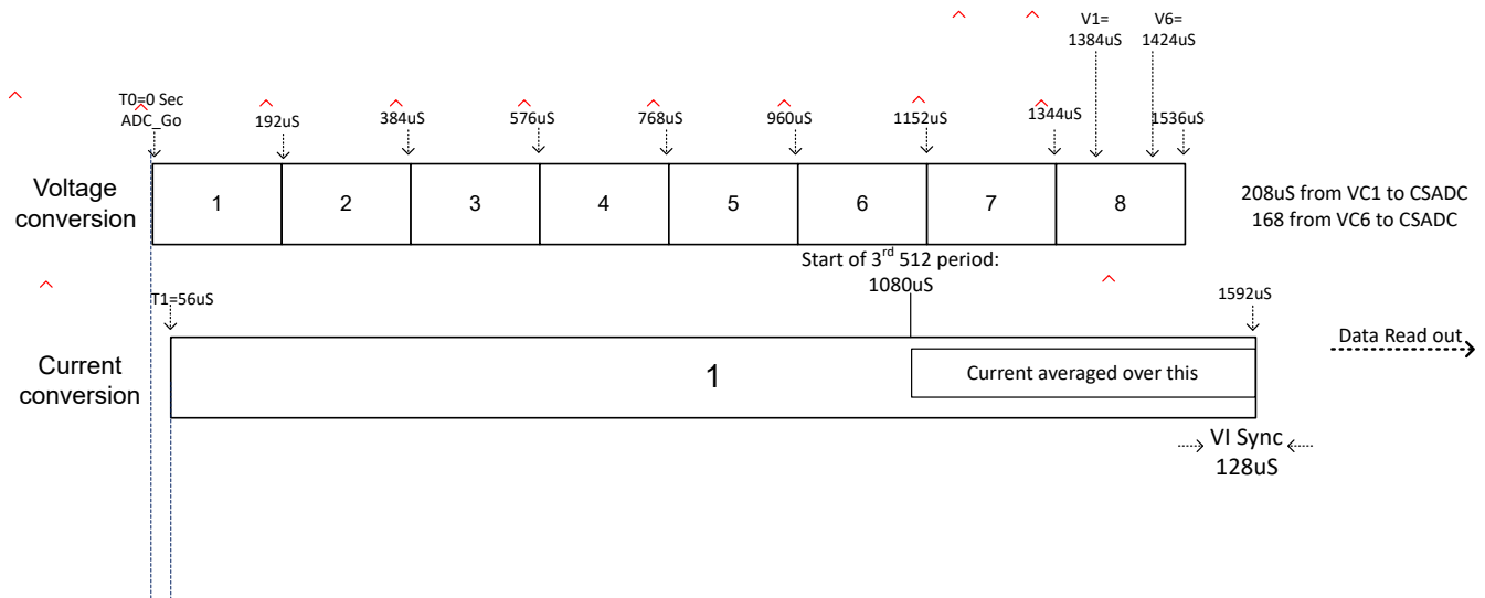
9-6. Single Conversion
