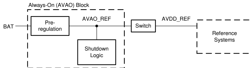
図 8-1. AVAO Block
