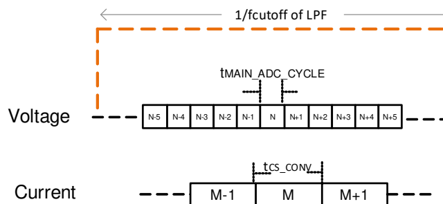
9-7. Effect of Voltage Low Pass Filter in Continuous Run Mode
