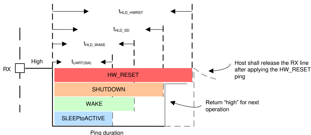
図 8-39. Communication Pings
