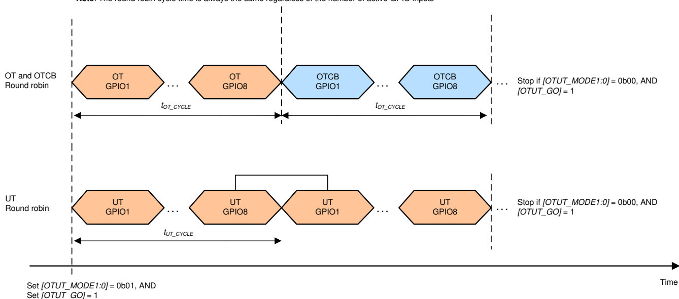
図 8-22. OT and UT Round Robin Modes
