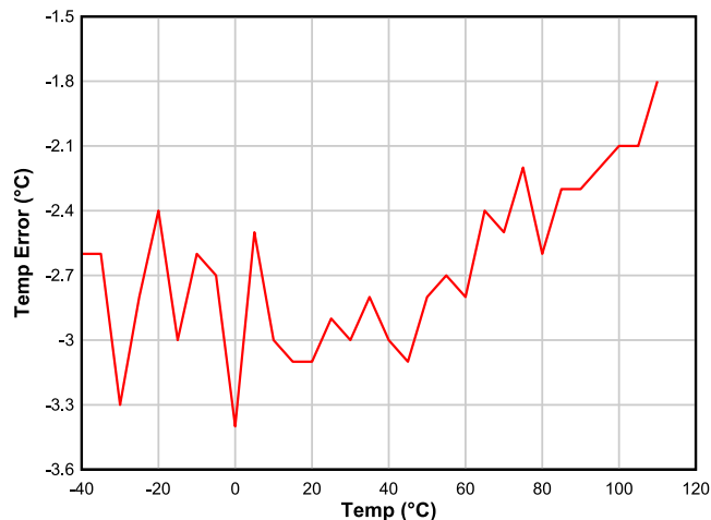
✎ 16-2. Thermistor Temperature Error
