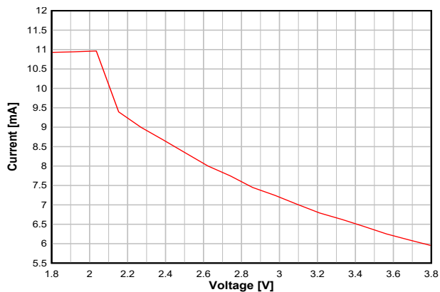
8-15. TX Current vs. Supply Voltage (VDD) (BLE 1 Mbps, 2.44 GHz, 0 dBm)
