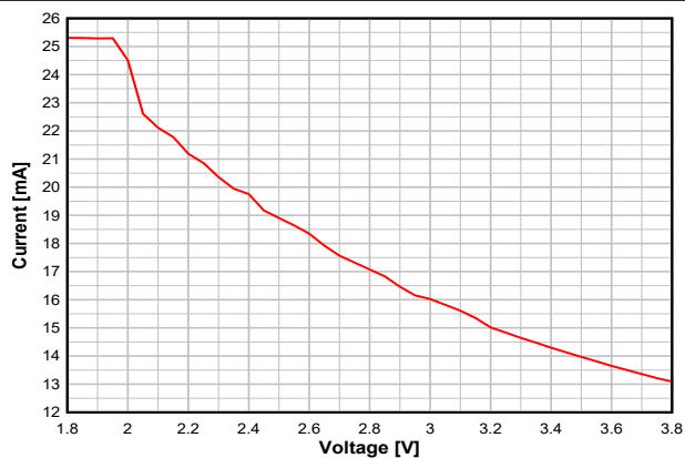
8-14. TX Current vs. Supply Voltage (VDD) (50 kbps, 868.3 MHz)
