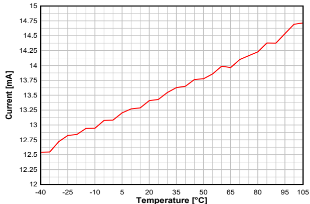
8-12. TX Current vs. Temperature (50 kbps, 868.3 MHz, VDD = 3.6 V)
