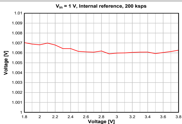
8-45. ADC Accuracy vs. Supply Voltage (VDDS)
