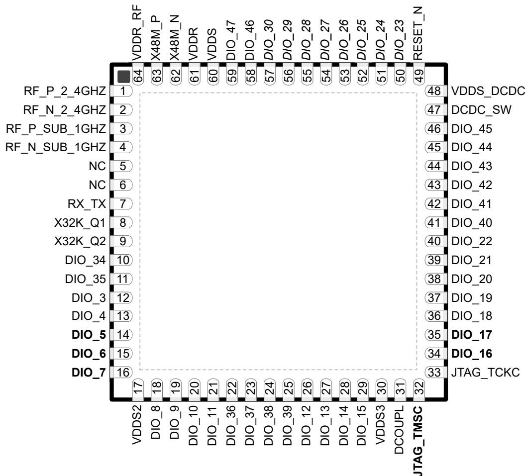
FIG 7-2. RSK (8 mm × 8 mm) Pinout, 0.4 mm Pitch (Top View)
