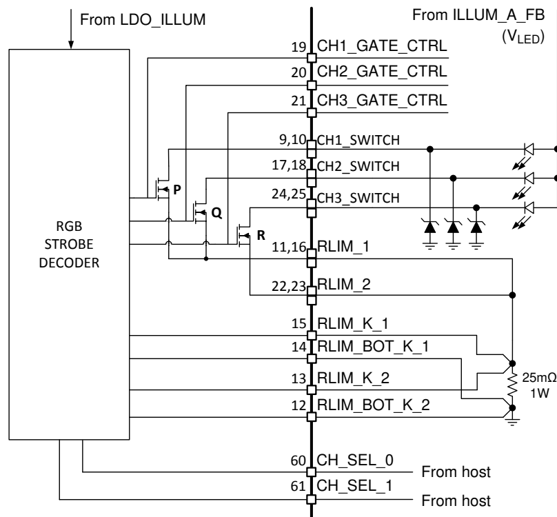
図 8-7. Switch Connection for a Common-Anode LED assembly
