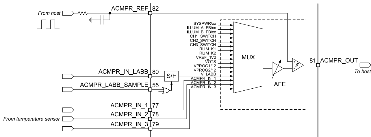
Figure 8-23. Measurement System
