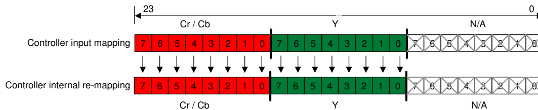
FIG 7-3. 16-Bit YCbCr-880 I/O Mapping
