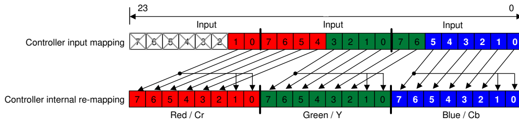
FIG 7-2. RGB-666 and YCbCr-666 I/O Mapping
