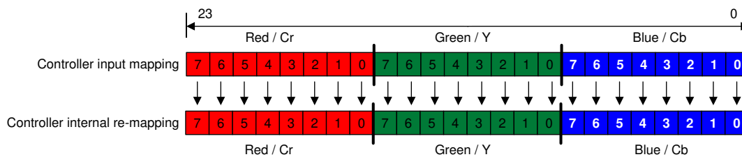
FIG 7-1. RGB-888 and YCbCr-888 I/O Mapping
