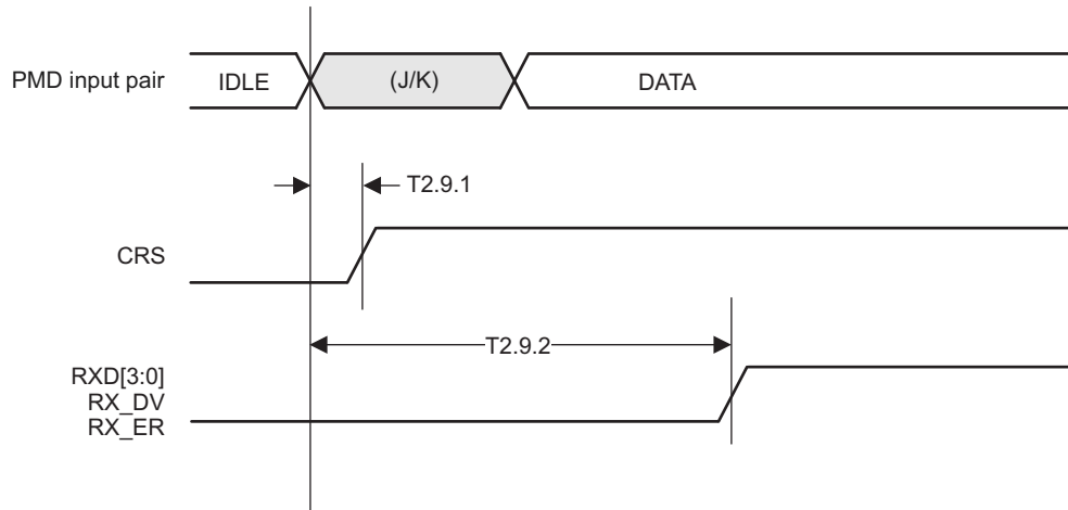
FIG 4-10. 100BASE-TX Receive Packet Latency Timing
