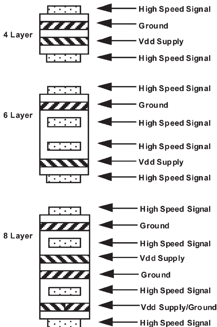
FIG 8-3. PCB Stripline Layer Stacking
