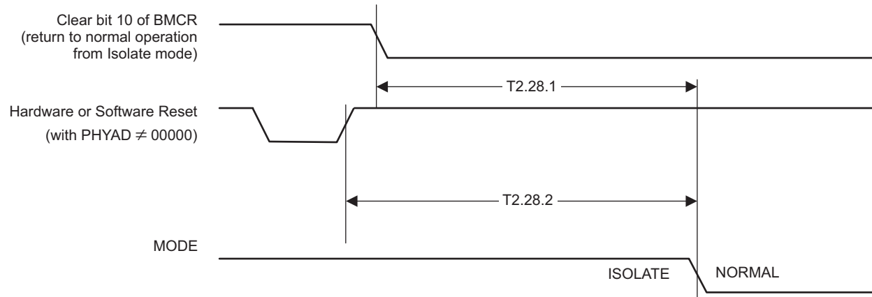
✎ 4-29. Isolation Timing
