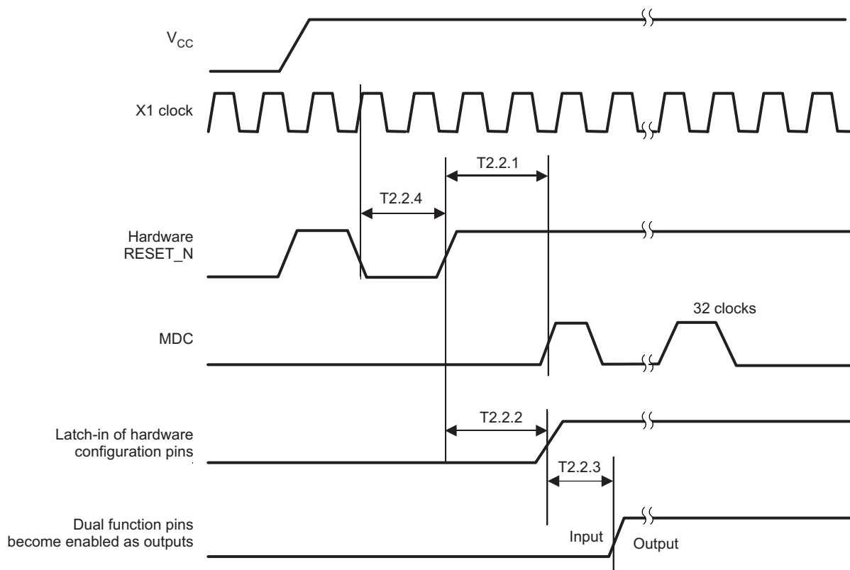
✎ 4-3. Reset Timing
