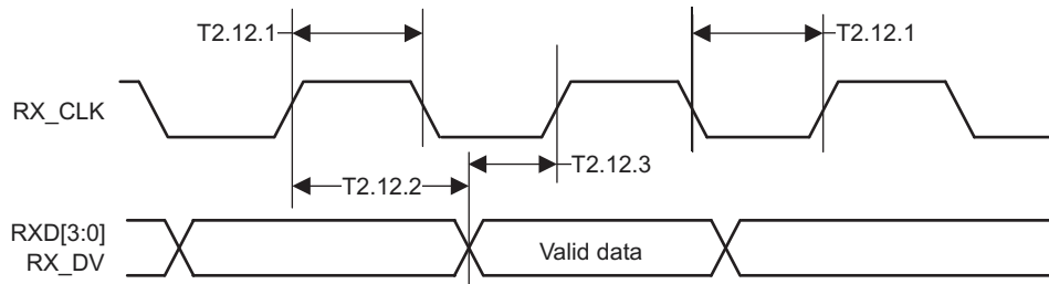
✎ 4-13. 10-Mbps MII Receive Timing
