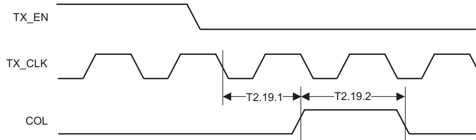
✎ 4-20. 10-Mbps Heartbeat Timing
