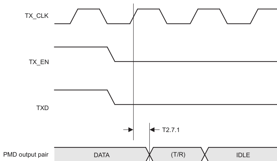
✎ 4-8. 100BASE-TX Transmit Packet Deassertion Timing
