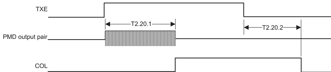
✎ 4-21. 10-Mbps Jabber Timing
