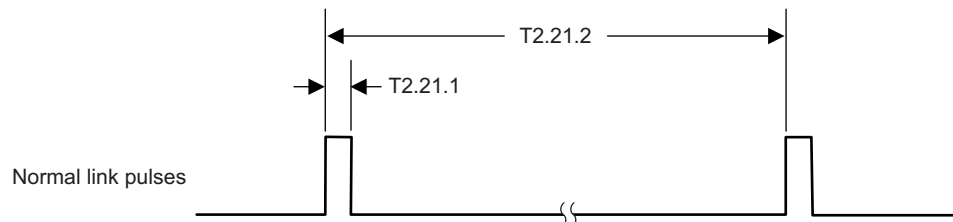
✎ 4-22. 10BASE-T Normal Link Pulse Timing
