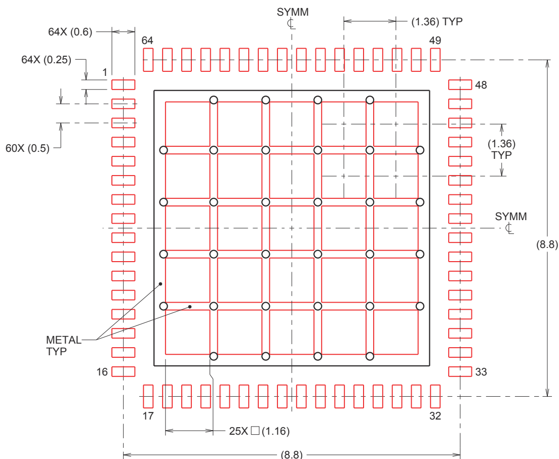
10-1. 64-Pin WQFN Stencil Example of Via and Opening Placement (Dimensions in mm)
