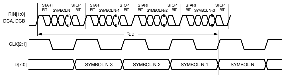
FIG 6-4. Latency Delay
