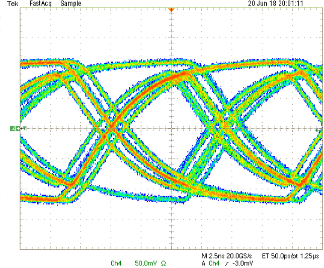
图 6-12. Back Channel Output Typical Waveform
