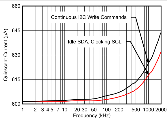
FIG 5-20. Active I_Q vs Clock Frequency
