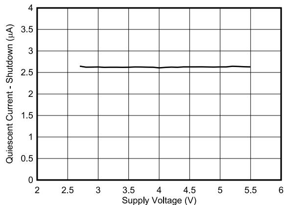
図 5-18. Shutdown I_Q vs Supply Voltage
