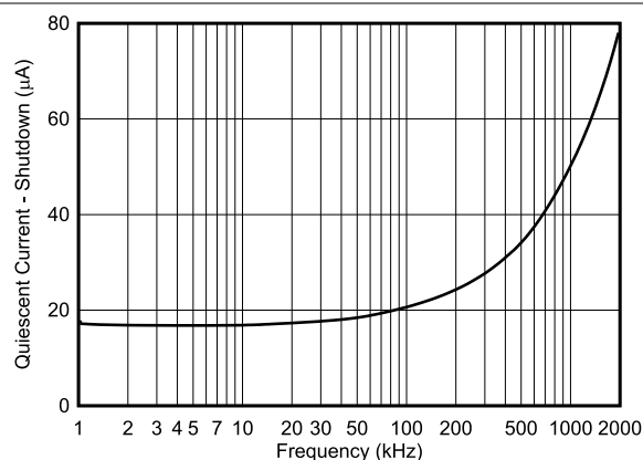
FIG 5-21. Shutdown I_Q vs Clock Frequency
