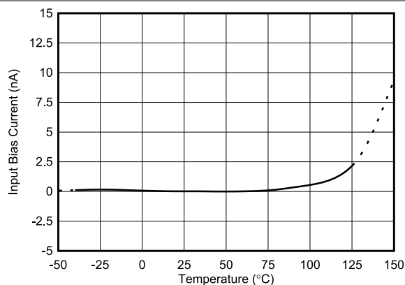
図 5-14. Input Bias Current vs Temperature
