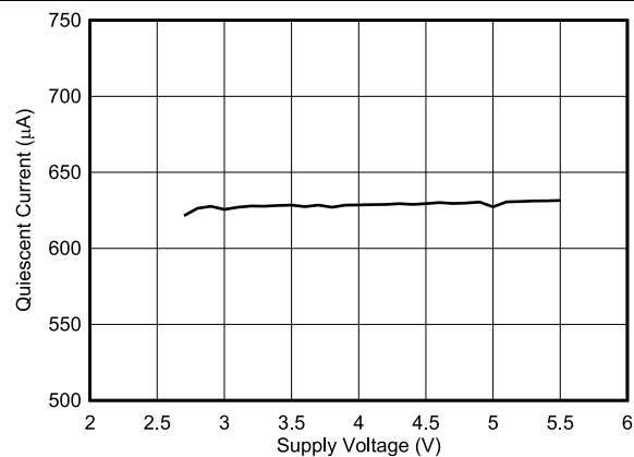
図 5-17. Active I_Q vs Supply Voltage
