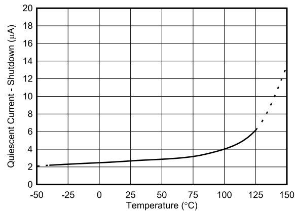
図 5-19. Shutdown I_Q vs Temperature
