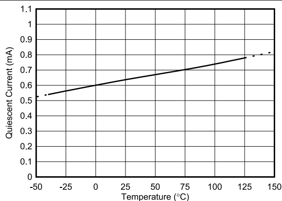
図 5-16. Active I_Q vs Temperature
