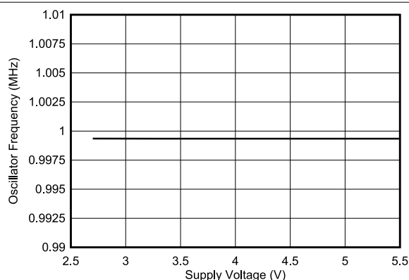
FIG 5-22. Internal Clock Frequency vs Power Supply
