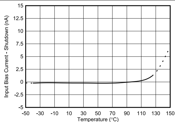
図 5-15. Input Bias Current vs Temperature, Shutdown
