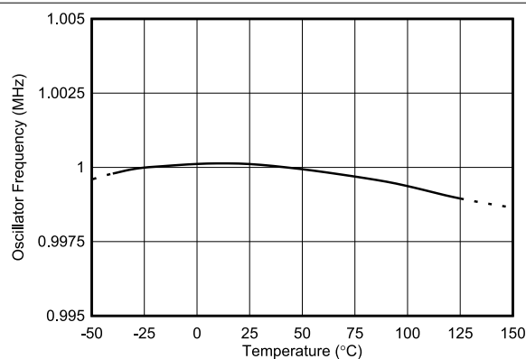
FIG 5-23. Internal Clock Frequency vs Temperature
