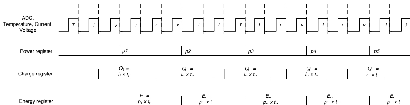
7-4. Power, Energy and Charge Calculation Scheme
