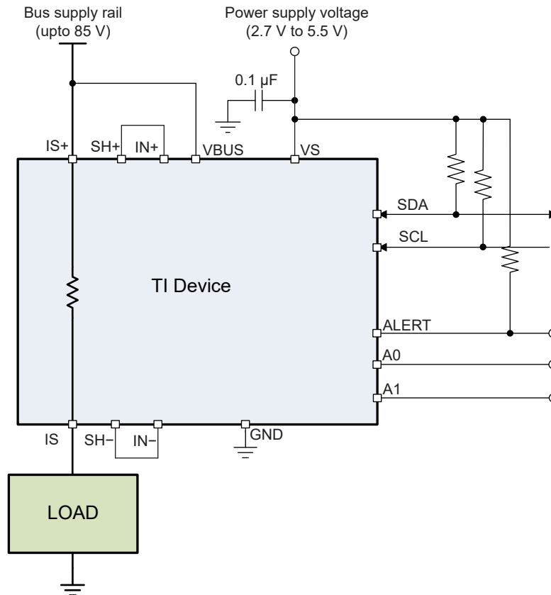
図 8-2. INA781 High-Side Sensing Application Diagram
