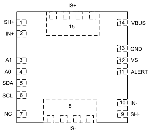
図 5-1. DEK Package 15-Pin WSON Top View
