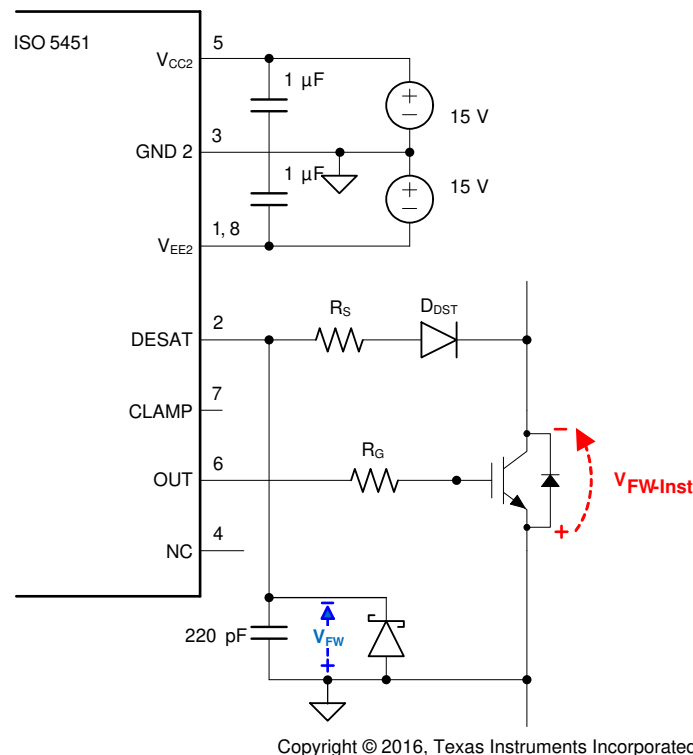
FIG 10-8. DESAT Pin Protection with Series Resistor and Schottky Diode
