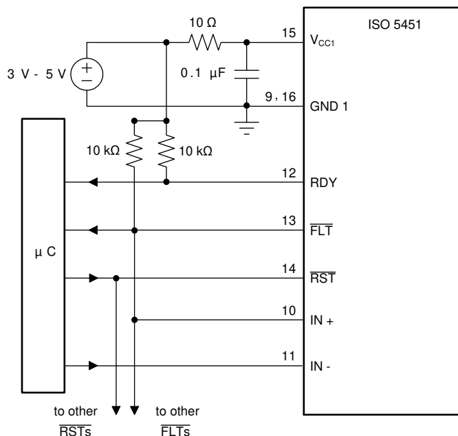
FIG 10-6. Global Shutdown With Inverting Input Configuration
