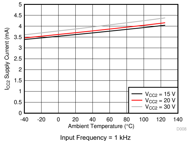
FIG 7-18. I_{CC2} Supply Current vs Temperature
