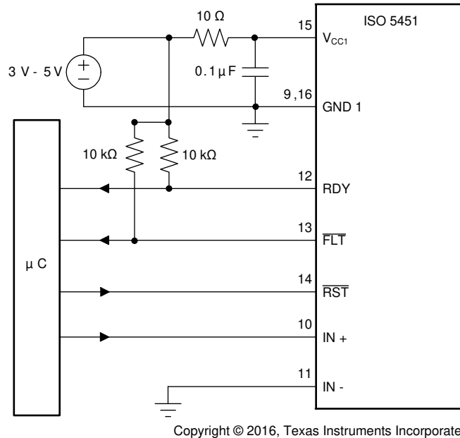
FIG 10-4. \overline{\text{FLT}} and RDY Pin Circuitry for High CMTI
