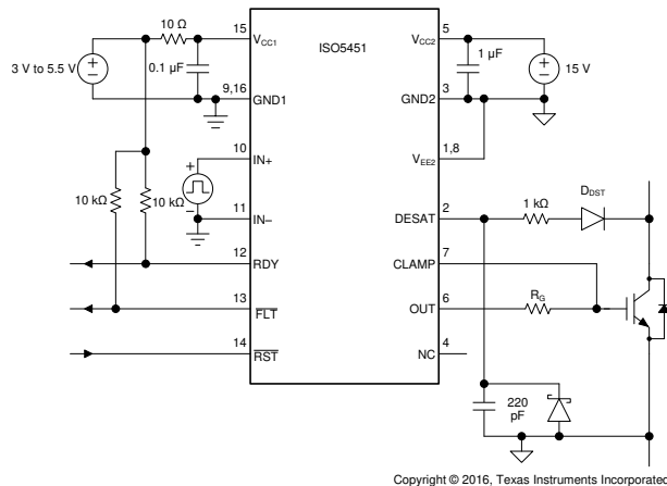
FIG 10-2. Unipolar Output Supply
