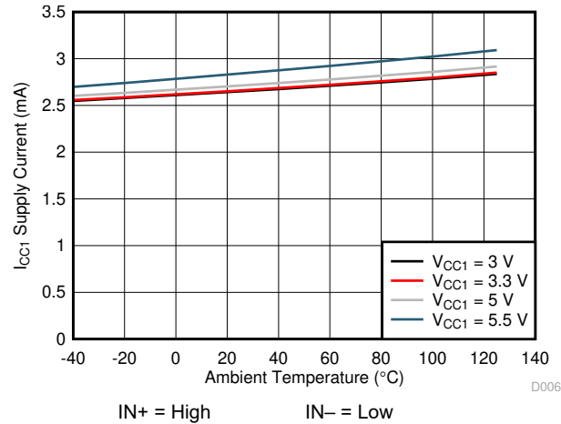
FIG 7-16. I_{CC1} Supply Current vs Temperature
