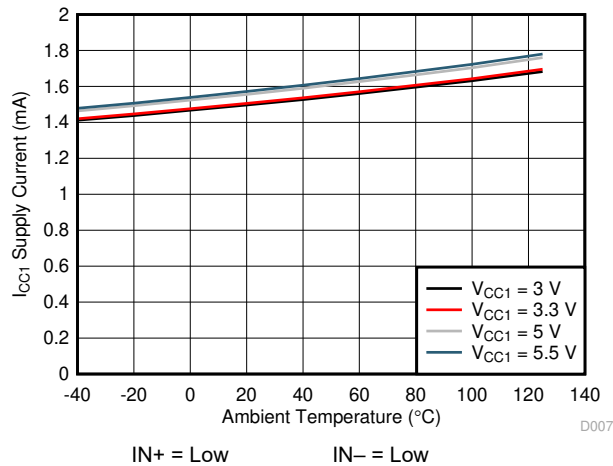
FIG 7-17. I_{CC1} Supply Current vs Temperature
