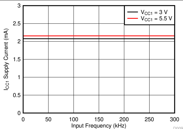
FIG 7-19. I_{CC1} Supply Current vs Input Frequency
