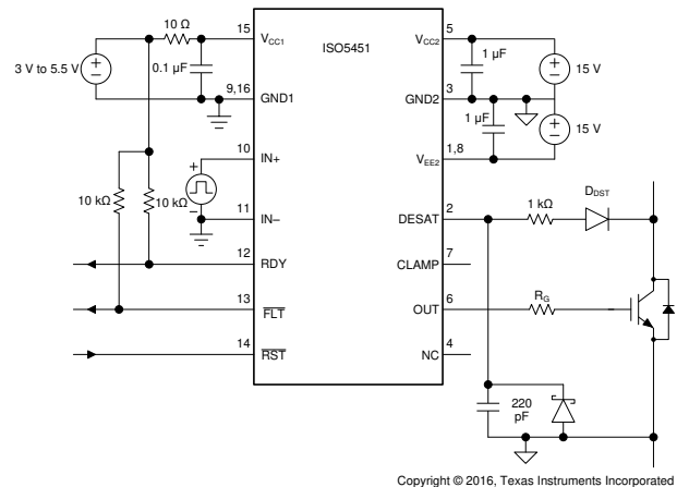
FIG 10-3. Bipolar Output Supply
