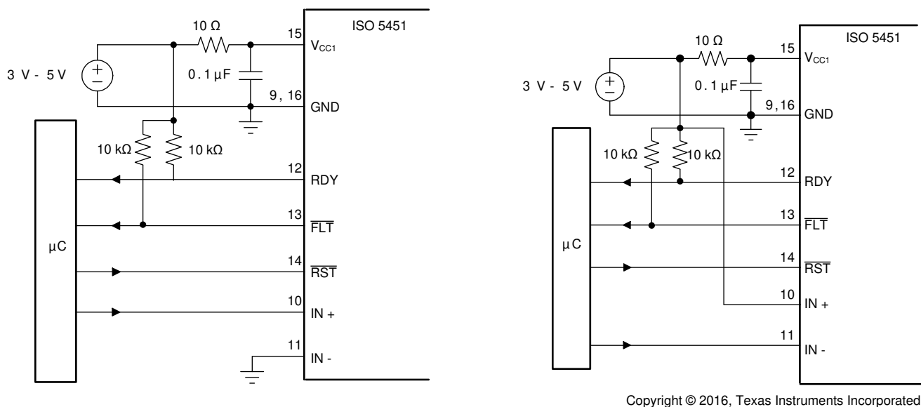
FIG 10-5. Local Shutdown and Reset for Noninverting (left) and Inverting Input Configuration (right)
