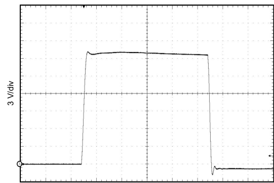
FIG 7-9. Output Transient Waveform
