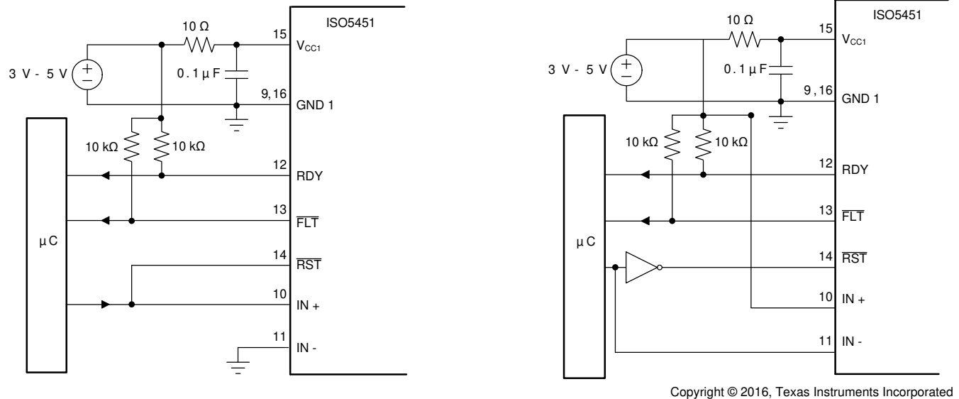
FIG 10-7. Auto Reset for Noninverting and Inverting Input Configuration
