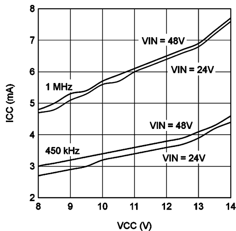
6-4. I_{CC} vs External V_{CC}
