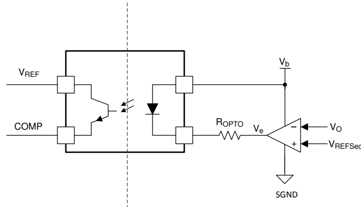
8-12. Opto-Coupler Interface
