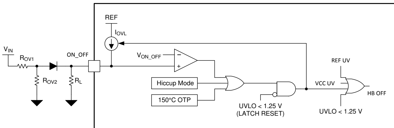
7-20. ON/OFF Pin Latch Function
