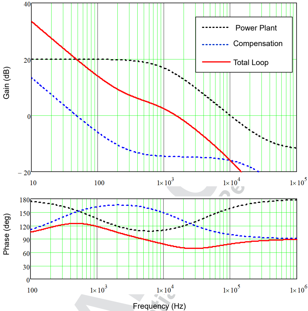
8-11. Bode Plots of the current loop
