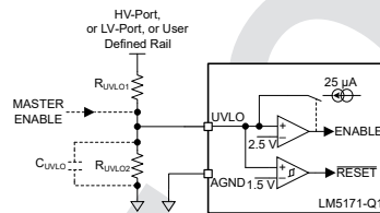
図 7-31. UVLO Programming
