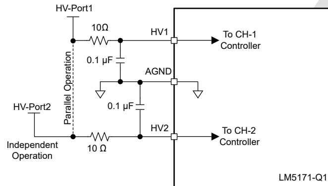
Figure 7-2. HV1 and HV2 Pins Configuration
