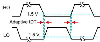
7-18. Adaptive Dead Time (Only One Channel is Shown)
