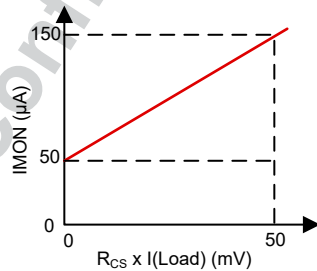
FIG 7-6. IMON Current Source vs Boost Load Current
