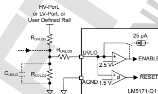
図 7-32. UVLO With Additional Hysteresis Programming
