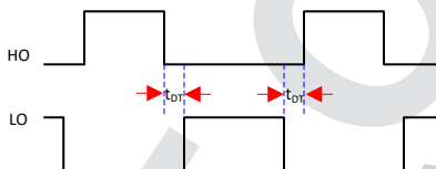
7-16. Gate Drive Dead Time (Only One Channel is Shown)
