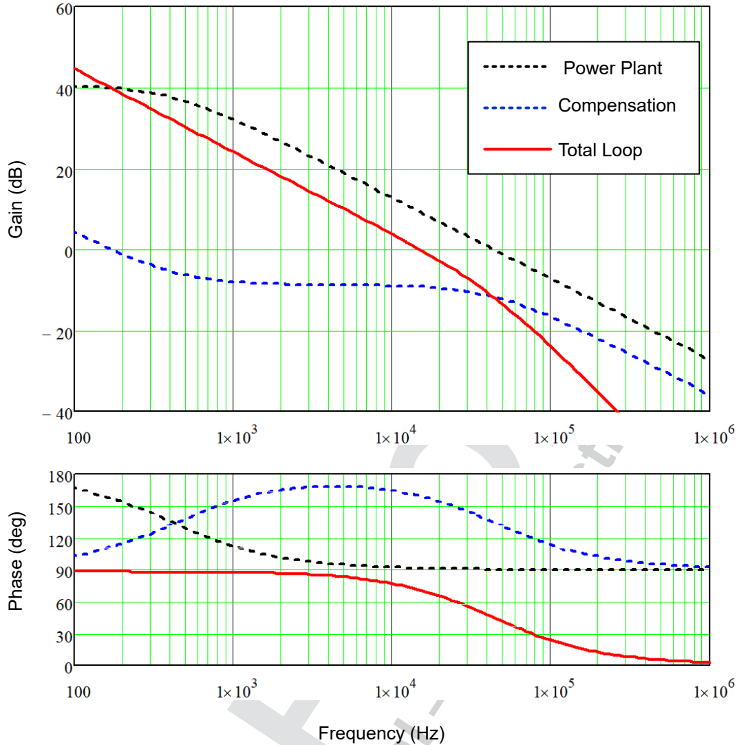
8-10. Bode Plots of the current loop
