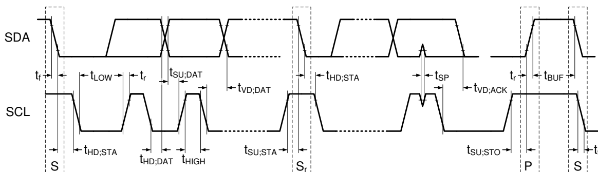
FIG 7-34. I 2 C Data Transmission Timing
