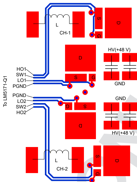
8-25. A Layout Example of MOSFET Gate Drive Routing
