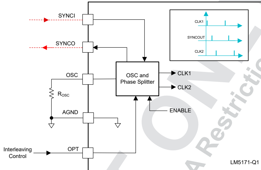
図 7-21. Oscillator and Interleaving Clock Programming
