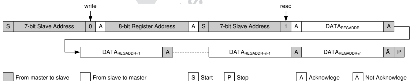
Figure 7-37. Sequential READ Starting From A Defined Register Address
