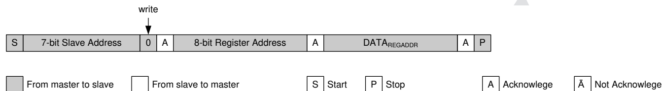
FIG 7-38. Single WRITE to Defined Register Address
