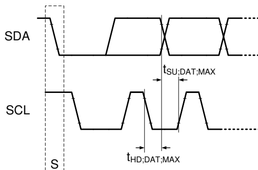
FIG 7-35. I 2 C Data Transmission Timing for maximum rise/fall times.
