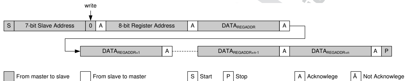
FIG 7-39. Sequential WRITE Starting At A Defined Register Address
