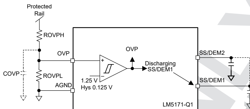
Figure 7-22. OVP for CH-1 or Multiphase Parallel Operation
