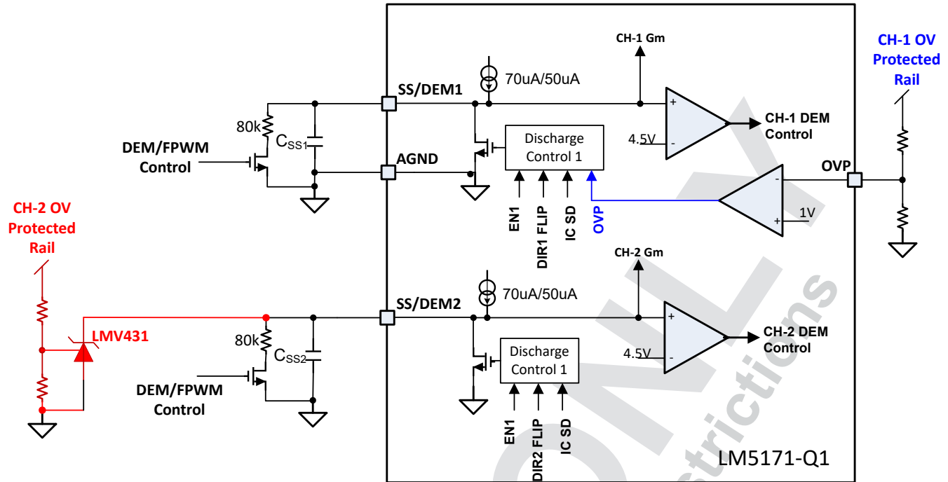
图 7-24. Independent Channel Operation OVP Implementation
