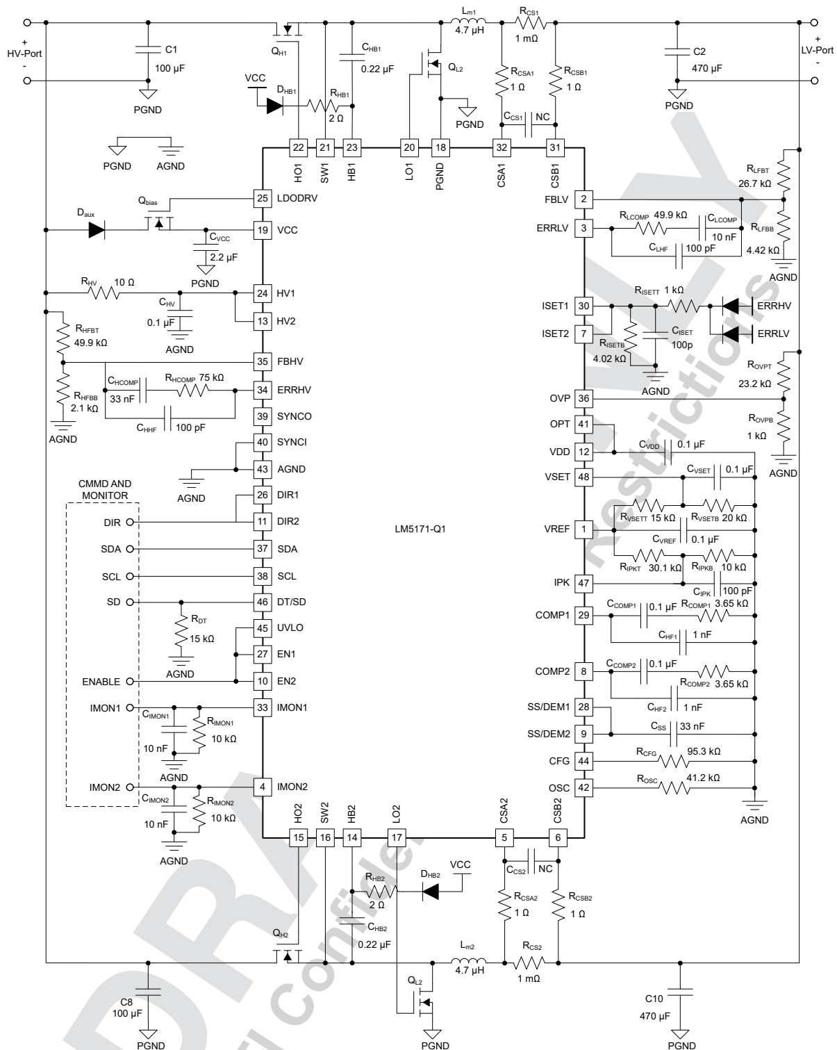
8-6. Schematic of the Example Dual-Phase Bidirectional Converter
