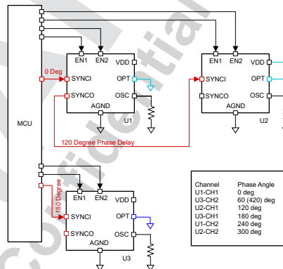
图 7-26. Six Phases 60° Interleaving Configuration using External Clock Shift
