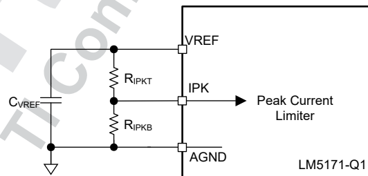
Figure 7-9. Cycle-by-Cycle Peak Current Limit Programming
