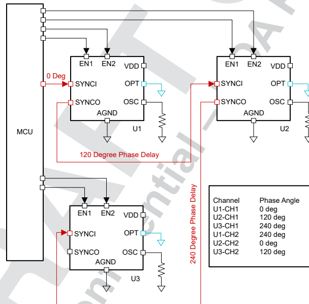
图 7-28. Six Phases 120° Interleaving Configuration using Internal Clock Shift
