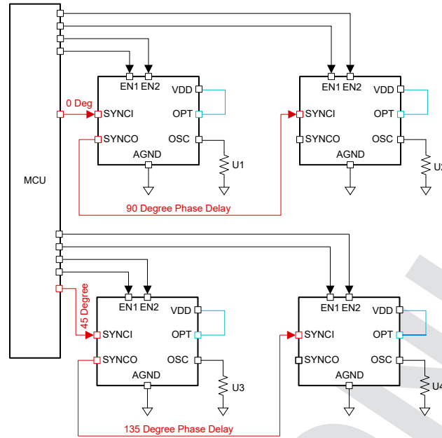
图 7-27. Eight Phases 45° Interleaving Configuration using External Clock Shift
