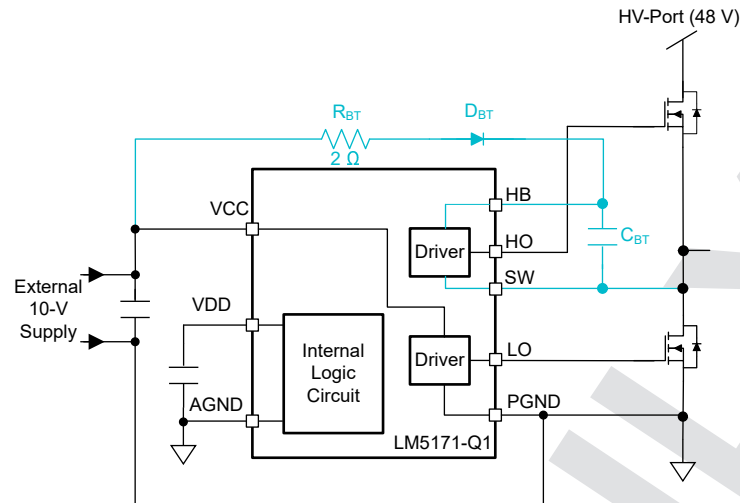
图 7-14. Bootstrap Circuit for High-Side Bias Supply (Only One Channel is Shown)
