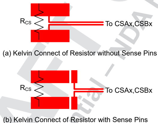
8-26. A Layout Example of Current Sense Routing
