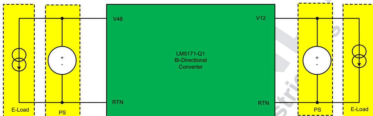
Figure 8-23. Emulated Dual Battery System With Bench Power Supplies and E-Loads
