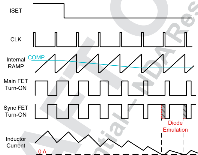
Figure 7-11. Diode Emulation Operation
