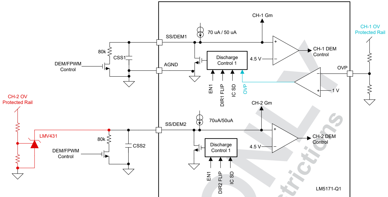
7-13. OVP Implementation for Independent Channel Operation
