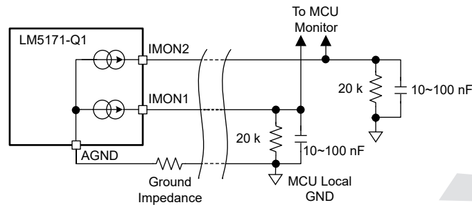
Figure 7-7. Channel Current Monitor
