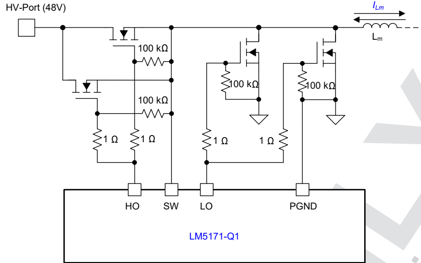
8-8. Paralleled MOSFET Configuration
