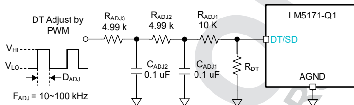
Figure 7-30. Dynamic Dead Time Adjustment b
