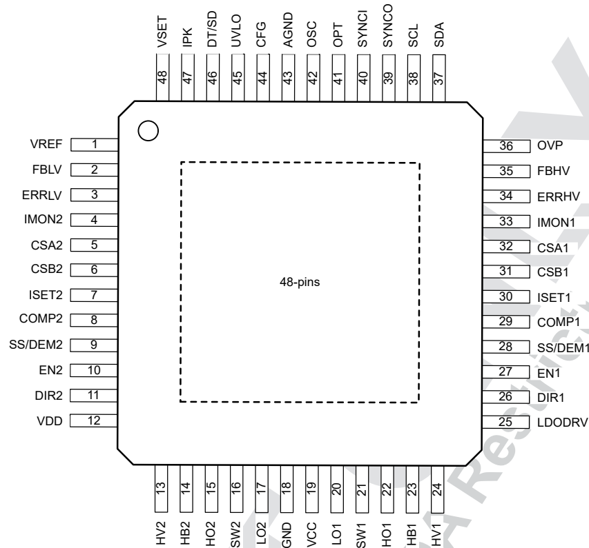
图 5-1. PHP Package 48-Pin TQFP Top View
