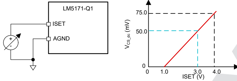
7-3. Analog Voltage Channel Current Programming
