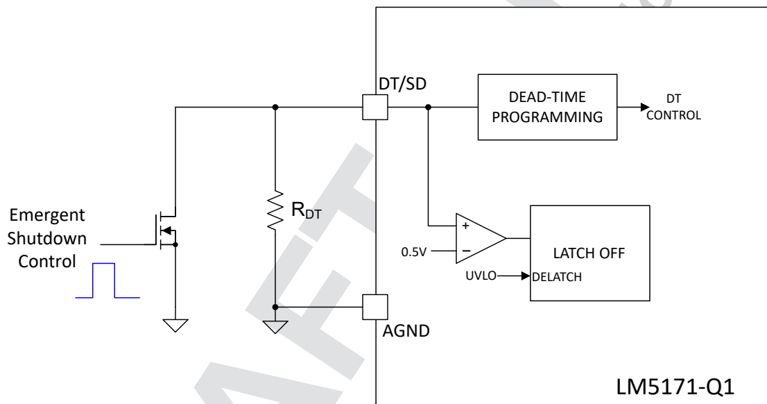
7-19. Emergent Latched Shutdown
