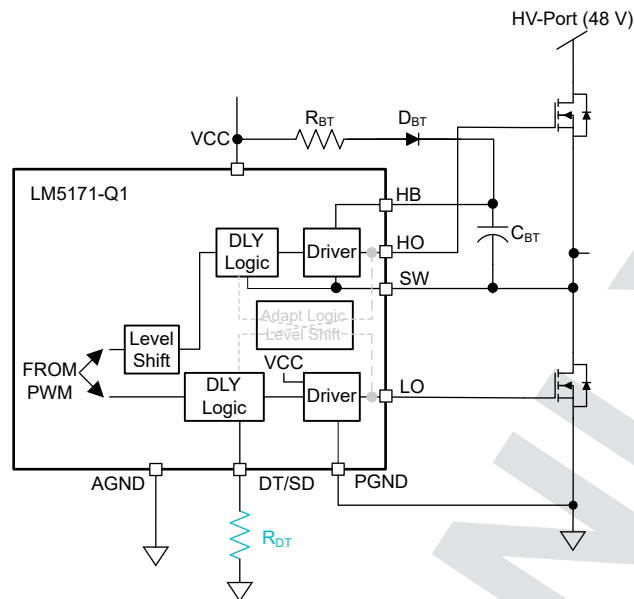
7-15. Dead Time Programming With DT Pin (Only One Channel is Shown)
