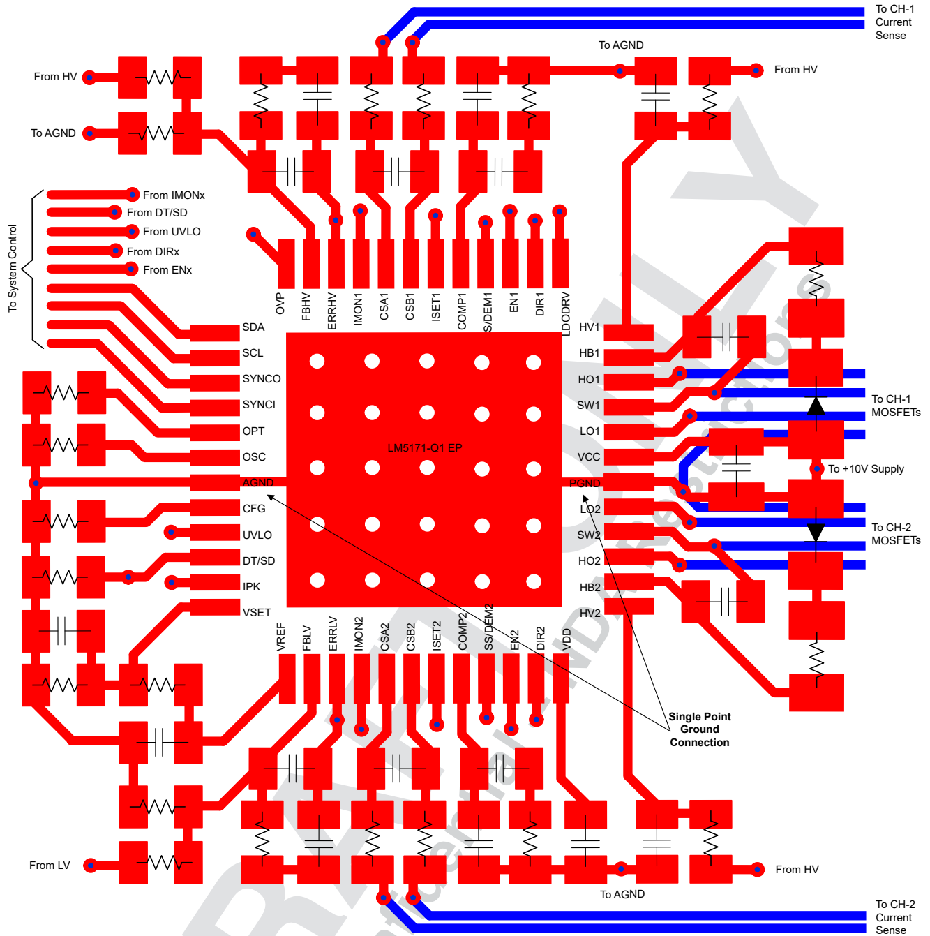
8-27. A Layout Example of LM5171-Q1 Critical Signal Routing
