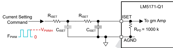
7-4. PWM Channel Current Programming
