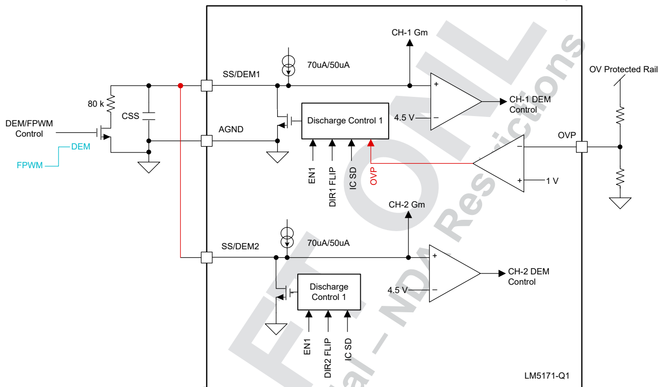
7-12. OVP Implementation for SS-DEM Pins Connection for Parallel Operation
