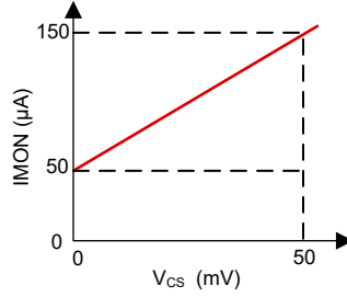
FIG 7-5. IMON Current Source vs Current Sense Voltage
