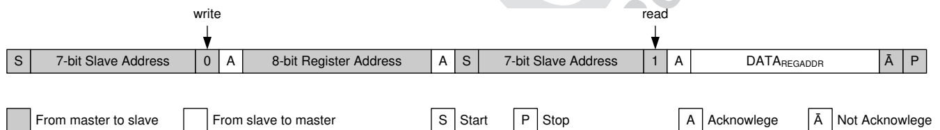
Figure 7-36. Single READ From a Defined Register Address
