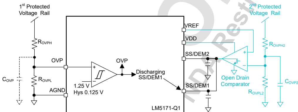
Figure 7-23. OVP for 2nd Protected Voltage Rail in Multiphase Parallel Operation
