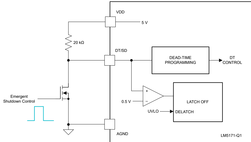
FIG 7-20. Emergent Latched Shutdown with Adaptive Dead-time Scheme
