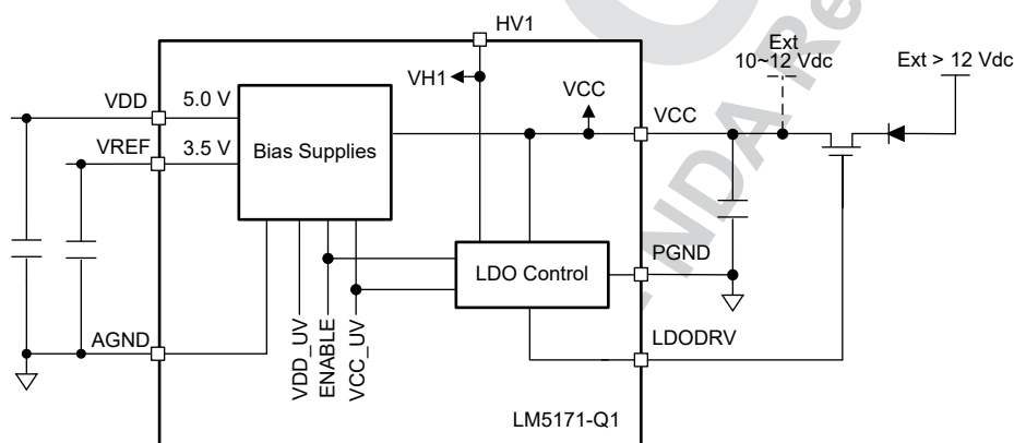
Figure 7-1. Bias Supplies Connections
