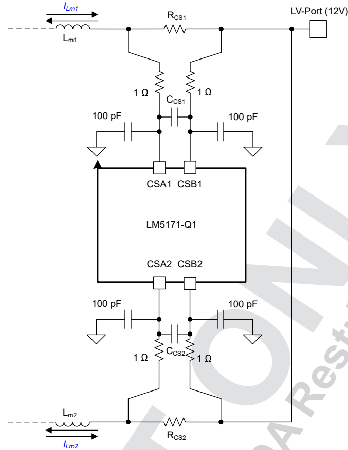
8-7. Current Sense With RC filter
