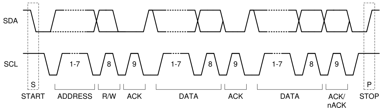
FIG 7-33. I 2 C START / STOP / ACKNOWLEDGE Protocol
