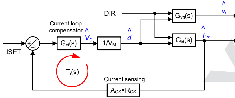
FIG 8-2. Current Loop Block Diagram
