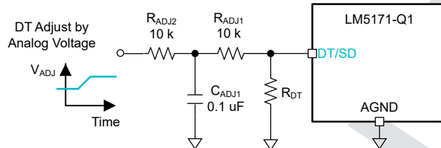
Figure 7-29. Dynamic Dead Time Adjustment A
