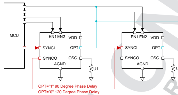
图 7-25. Three or Four Phases Interchangeable Configuration
