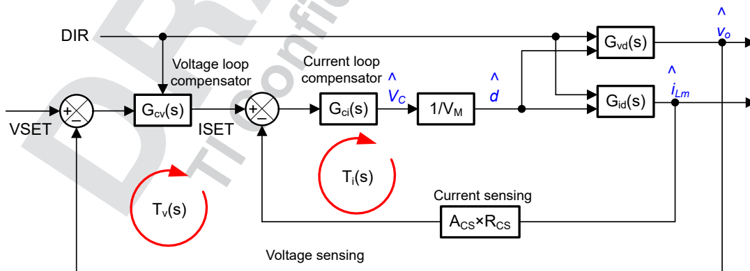
图 8-4. Voltage Loop and Current Loop Block Diagram
