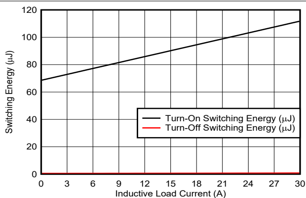
7-10. Half-Bridge Switching Energy vs Inductive Load Current
