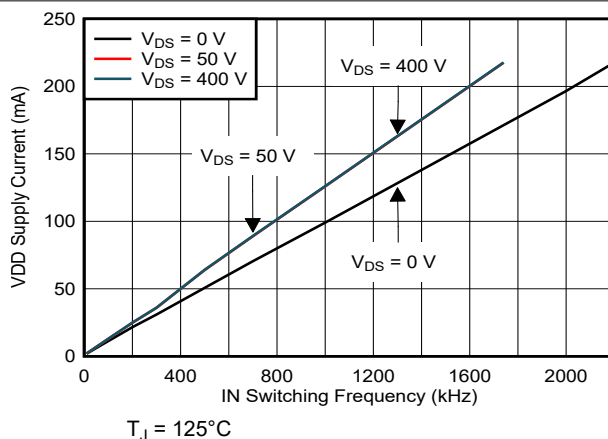
7-8. VDD Supply Current vs IN Switching Frequency
