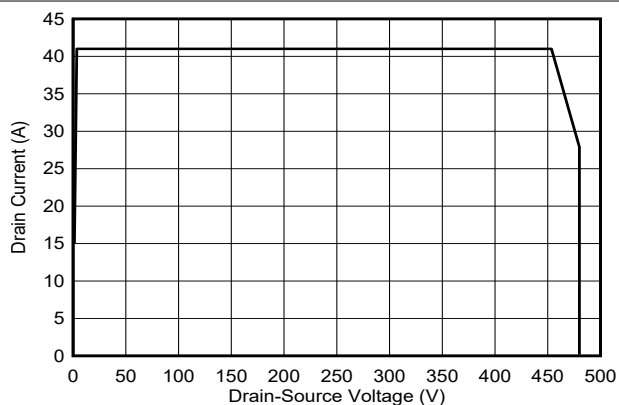
Figure 7-12. Repetitive Safe Operation Area
