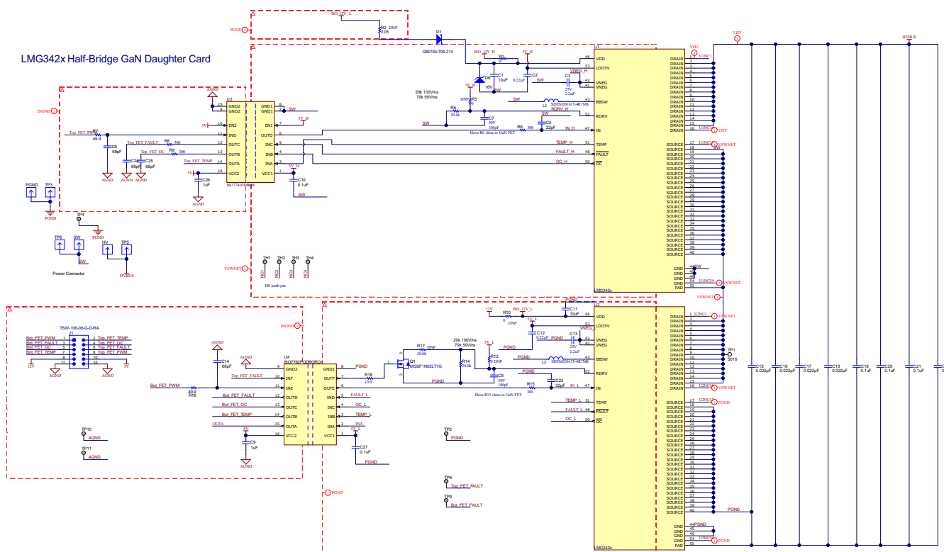
FIG 10-1. Typical Half-Bridge Application
