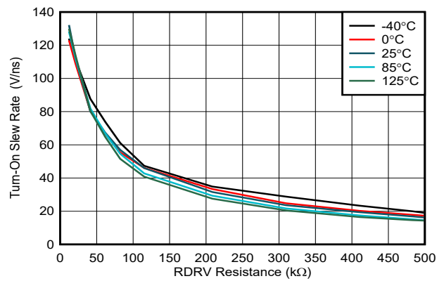
7-4. Turn-On Slew Rate vs Drive Strength Resistance
