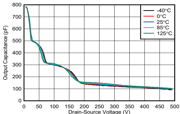
Figure 7-8. Output Capacitance vs Drain-Source Voltage
