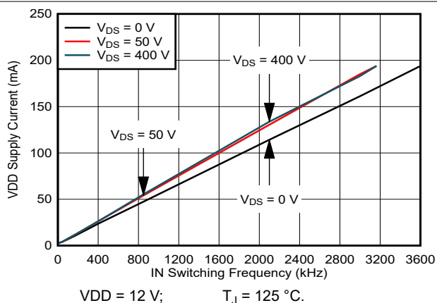
Figure 7-10. VDD Supply Current vs IN Switching Frequency
