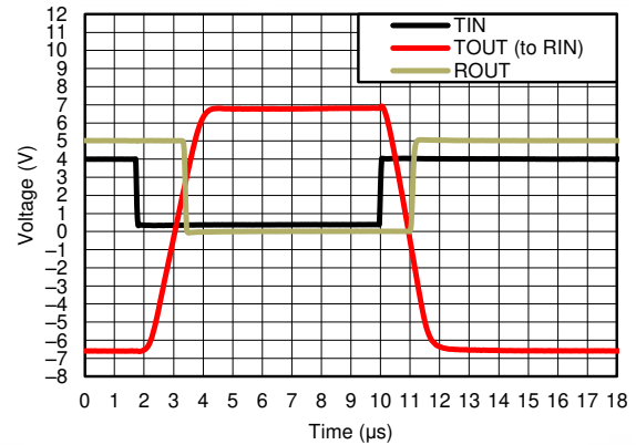
図 8-3. Driver to Receiver Loopback Timing Waveform
