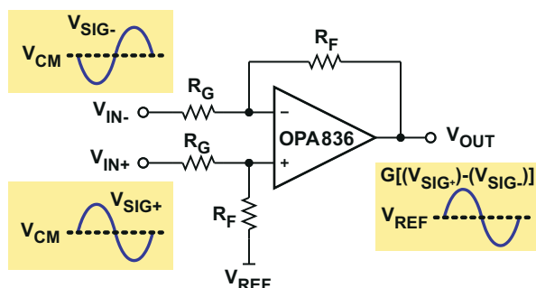
9-4. Differential to Single-Ended Amplifier
