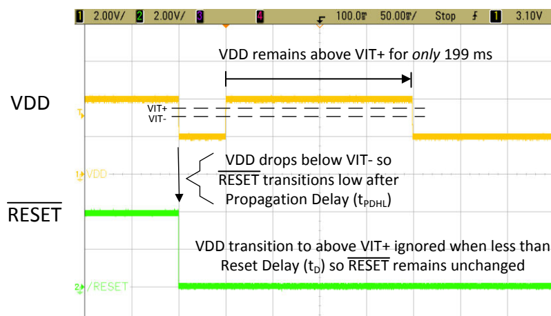
図 8-2. Glitch Immunity when VDD Rises Above V_{IT+} for Less than RESET Delay (TLV803EA29)
