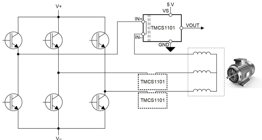
☒ 10-2. Inline Motor Phase Current Sensing
