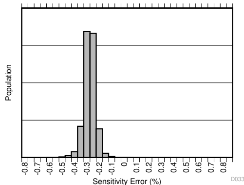
TMCS1101AxU
