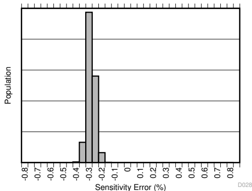
TMCS1101AxB
