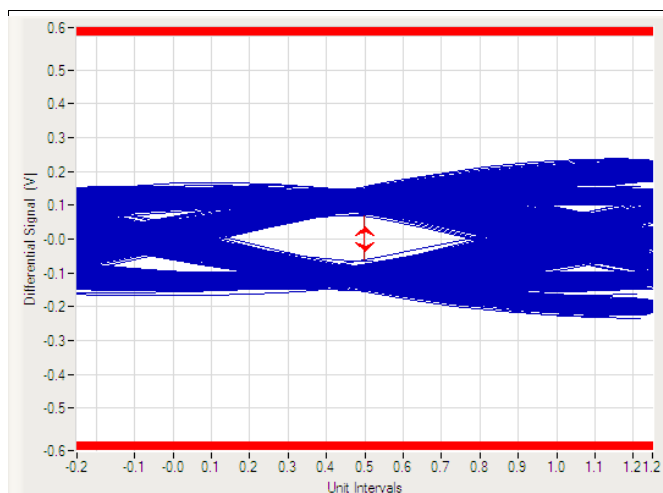
Figure 12. USB3.1 Gen 2 10-Gbps Eye Diagram (Bare Board)
