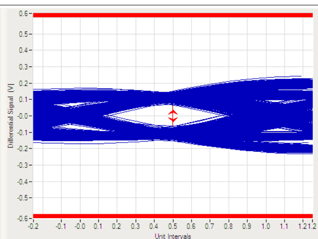
Figure 13. USB3.1 Gen 2 10-Gbps Eye Diagram (with TPD1E01B04DPL)
