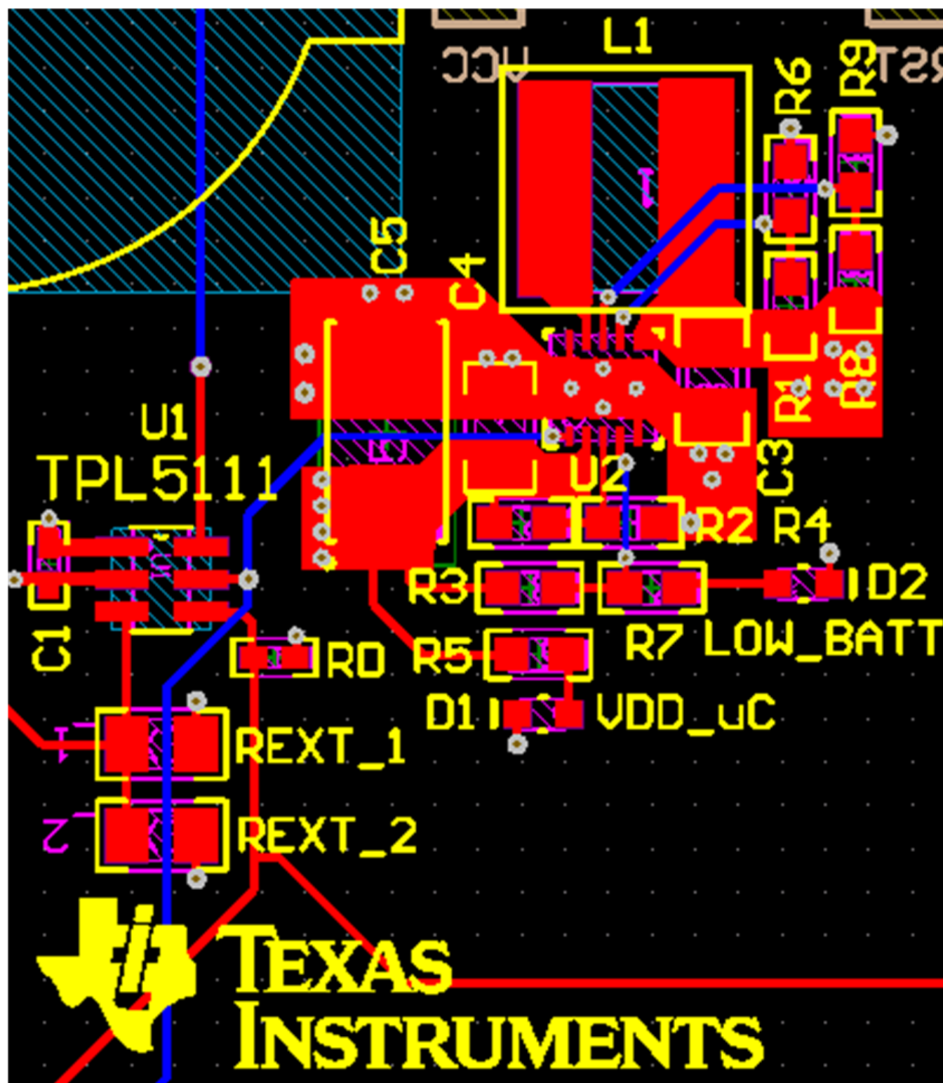
Figure 16. Layout
