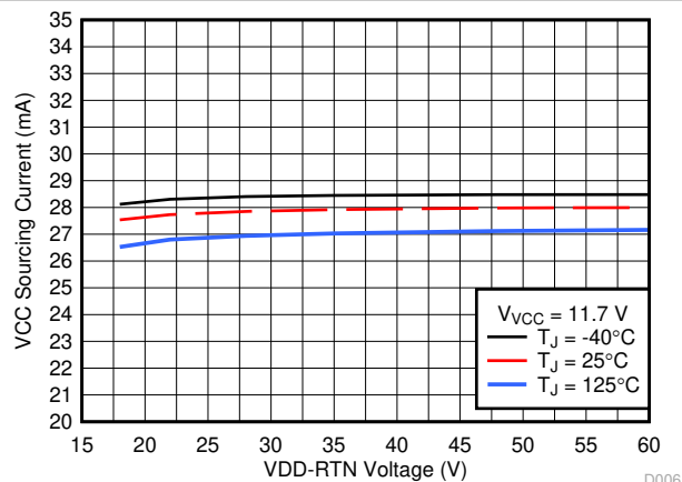
Figure 7-6. Converter Startup Current vs VDD Input Voltage
