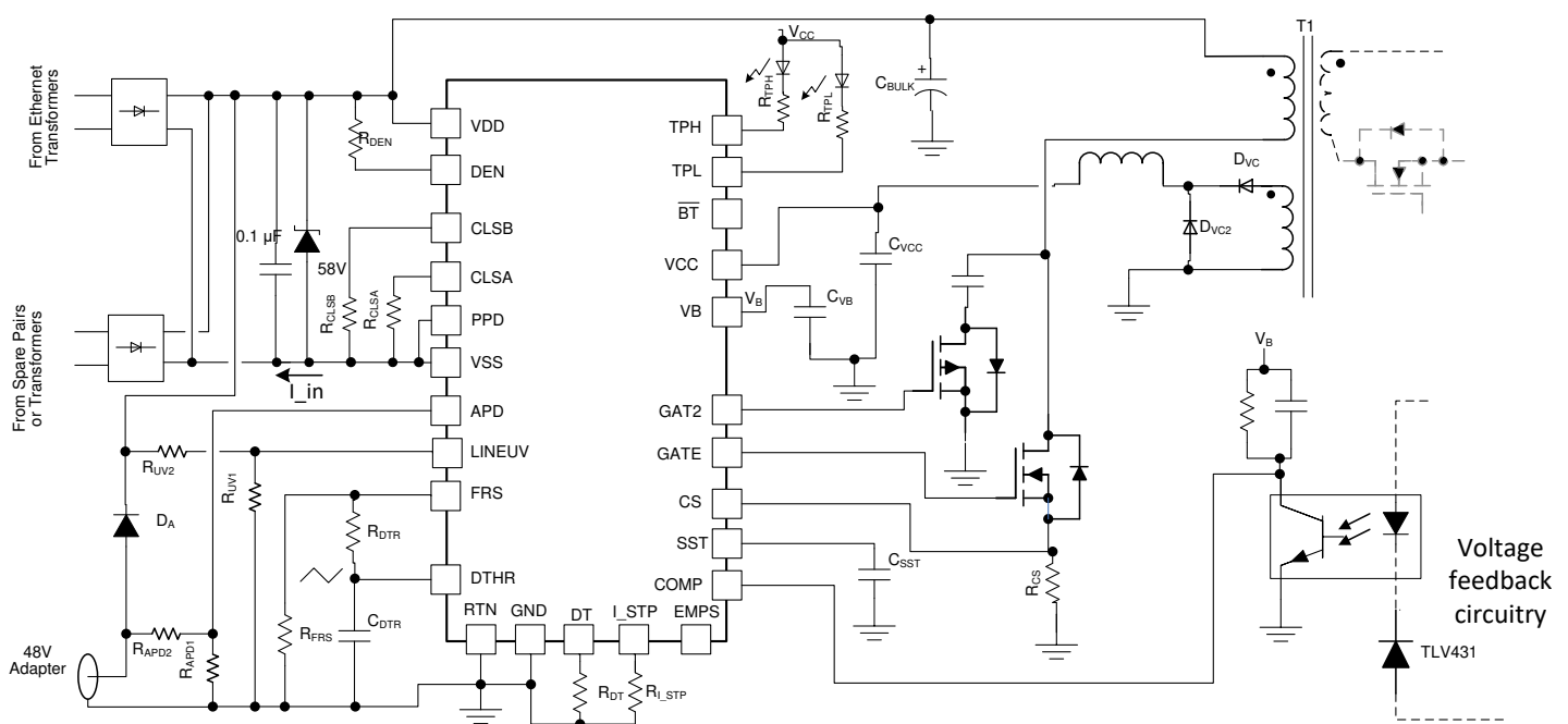
❏ 9-1. Basic TPS23730 Implementation
