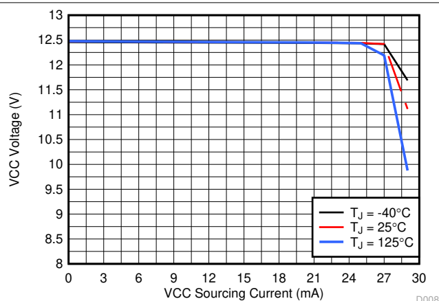
7-8. Converter Startup Voltage vs Current
