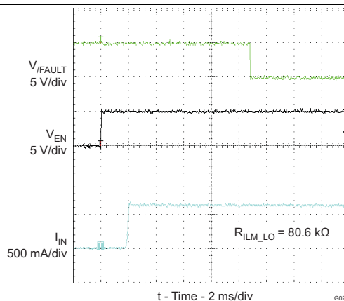
Figure 20. Device Enabled Into Short Circuit
