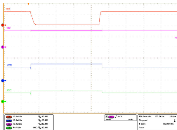
9-16. TPS259480x Power MUX - Switchover Between Primary and Auxiliary Supplies
