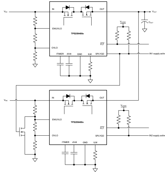
図 9-18. Priority Power MUXing With 2 × TPS25948x - Option 3
