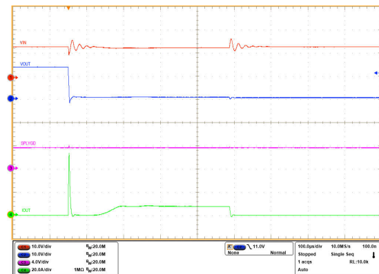
図 7-34. Transient Overcurrent Blanking Timer Response
