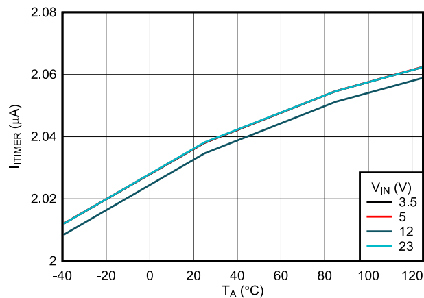
図 7-23. ITIMER Discharge Current vs Temperature
