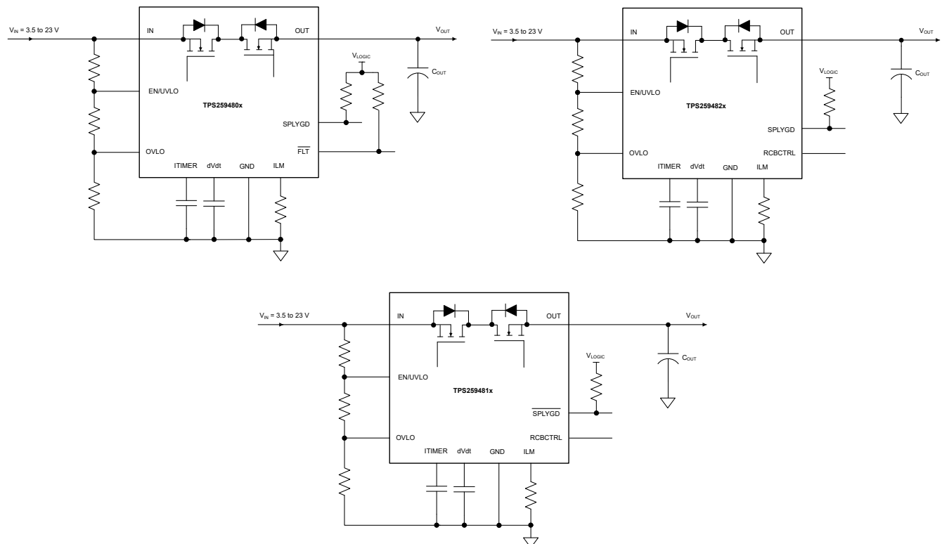
図 9-1. Single Device, Self-Controlled
