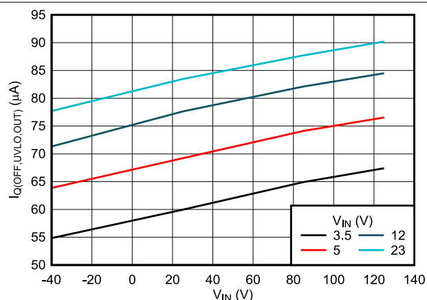
図 7-6. OUT OFF State (UVLO) Current vs Temperature
