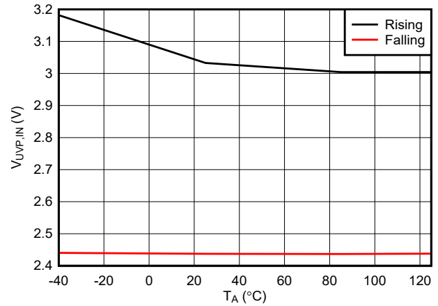
図 7-8. IN Undervoltage Threshold vs Temperature
