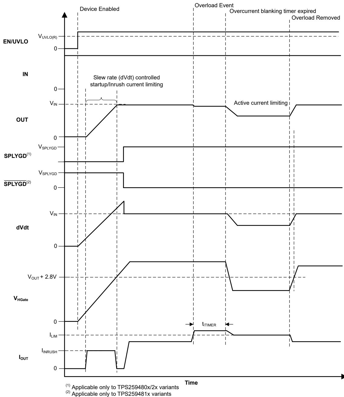
8-15. TPS25948xx SPLYGD Behavior
