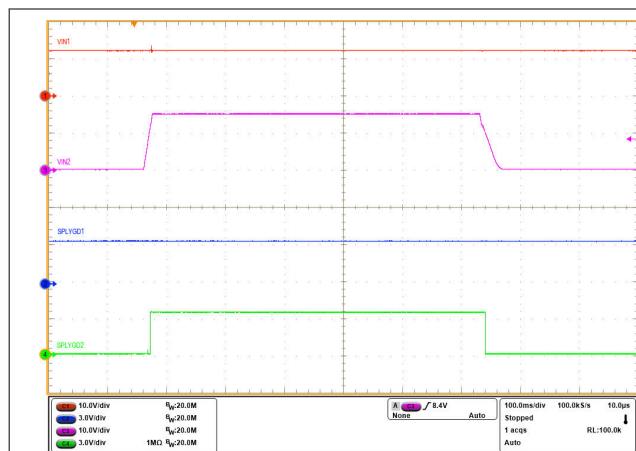
☒ 9-12. Active ORing Response
