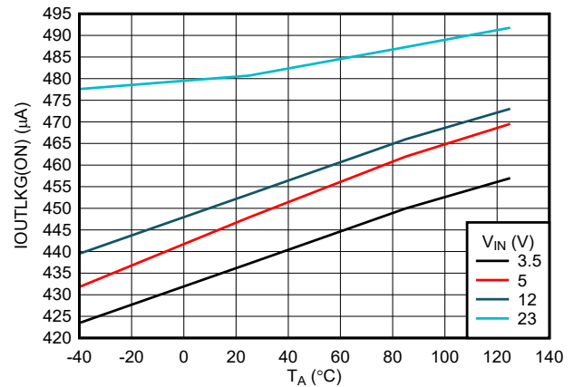
図 7-20. OUT Leakage Current During ON-State Reverse Current Blocking
