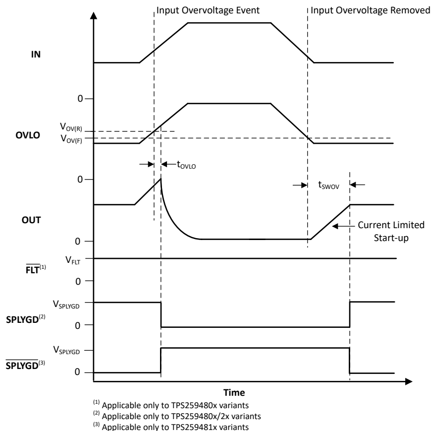
8-6. TPS25948xx Overvoltage Lockout and Recovery
