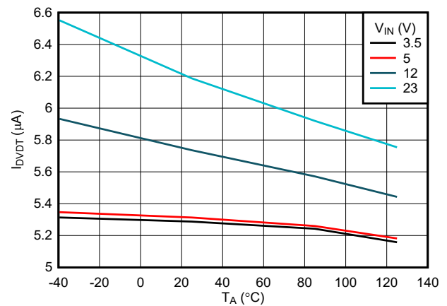
図 7-24. DVDT Charging Current vs Temperature
