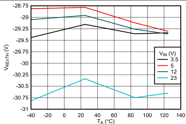
Figure 7-18. RCB - Reverse Comparator Threshold vs Temperature
