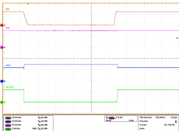
9-15. TPS259480x Power MUX - Switchover Between Primary and Auxiliary Supplies
