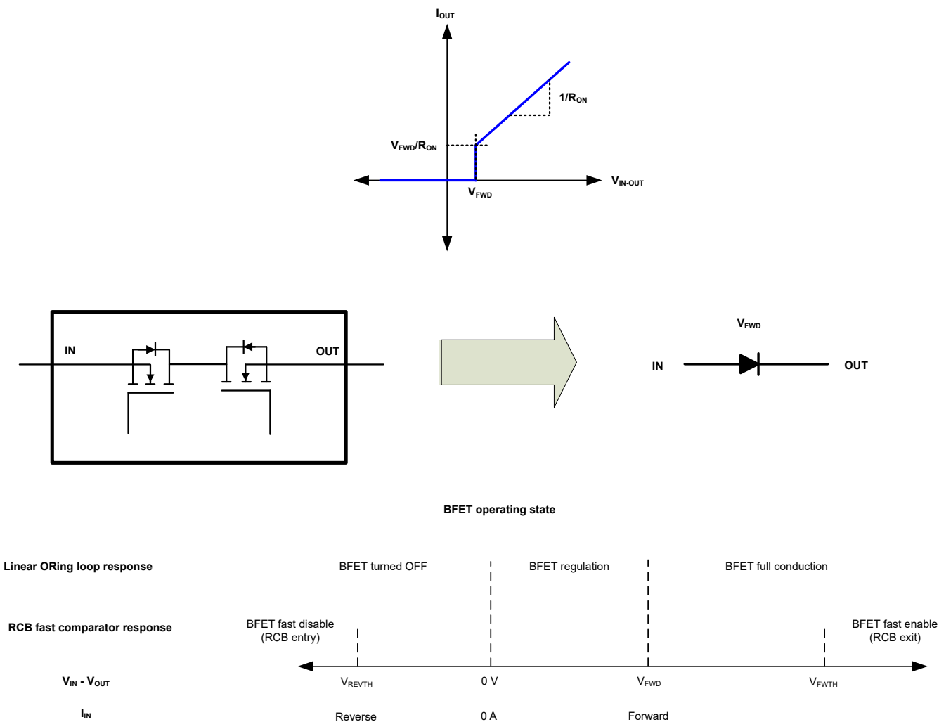
図 8-11. Reverse Current Blocking Response
