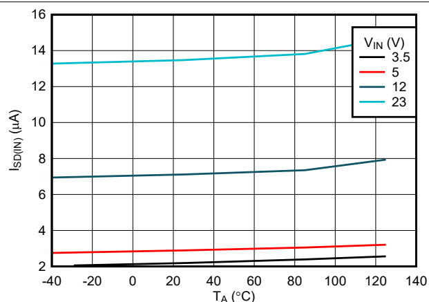
図 7-4. IN Shutdown Current vs Temperature
