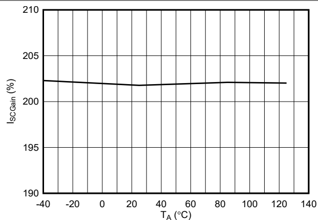
Figure 7-14. Steady State Scalable Fast-Trip Threshold: Current Limit Threshold ( I_{ILM} ) Ratio vs Temperature (TPS259480x/2x)
