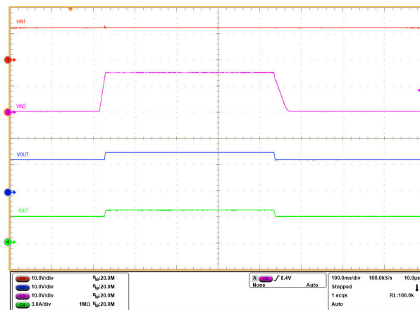
Figure 9-13. Active ORing Response
