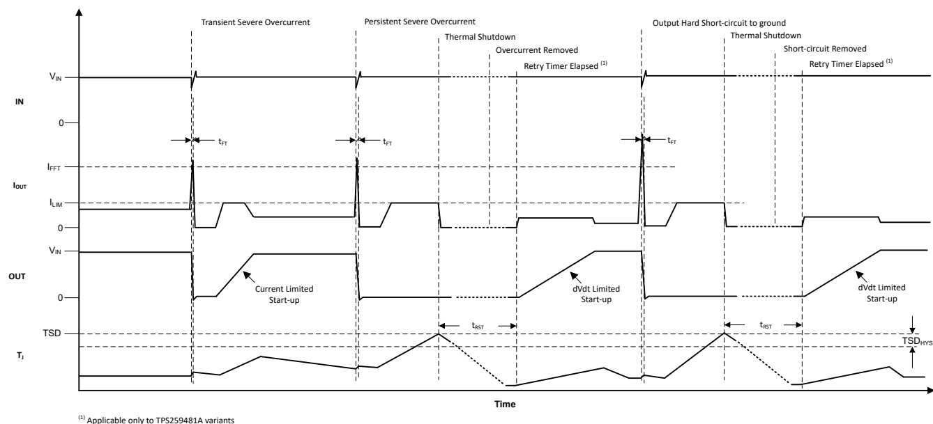
8-9. TPS259481x Short-Circuit Response
