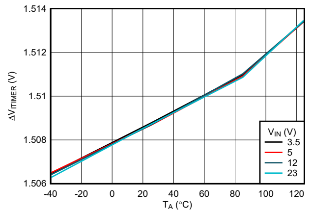
図 7-22. ITIMER Discharge Differential Voltage Threshold vs Temperature
