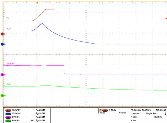
図 7-31. Inrush Current With Resistive and Capacitive Load
