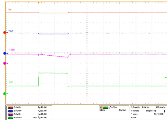
図 7-32. Inrush Current With Resistive and Capacitive Load
