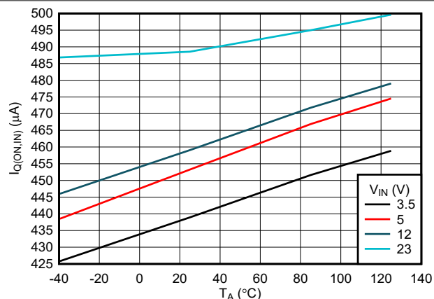
図 7-2. IN Quiescent Current vs Temperature
