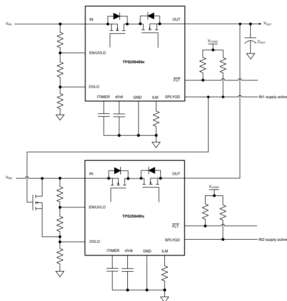
☒ 9-17. Priority Power MUXing With 2 × TPS259480x - Option 2
