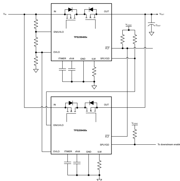
9-19. Two Devices Connected in Parallel for Higher Steady State Current Capability
