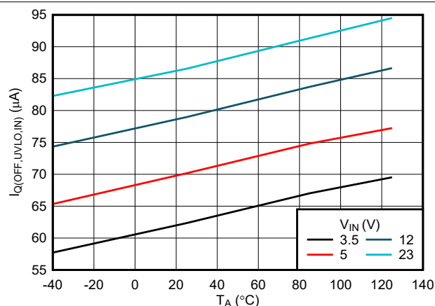
図 7-3. IN OFF state (UVLO) current vs Temperature
