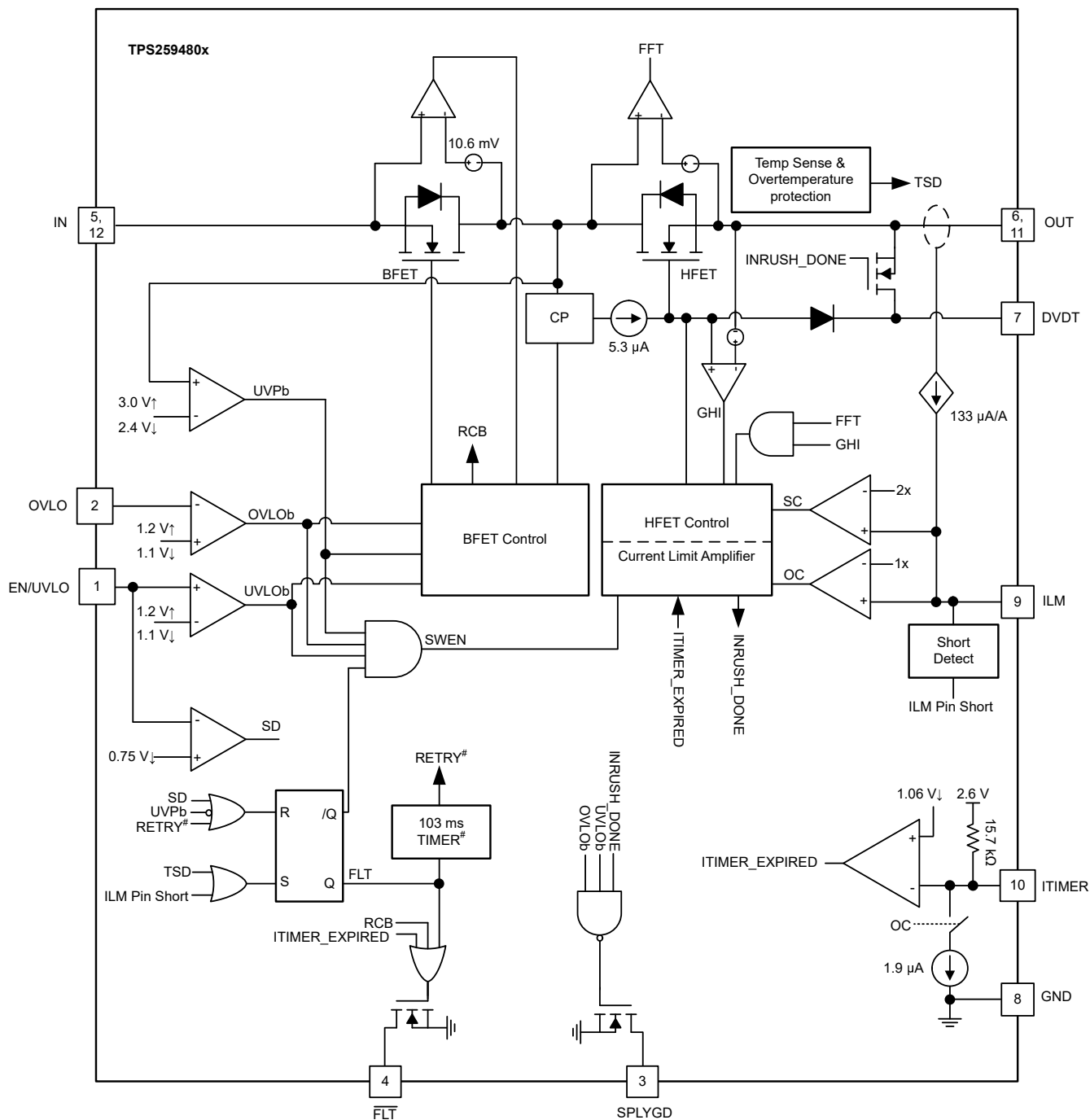
図 8-1. TPS259480x Block Diagram
