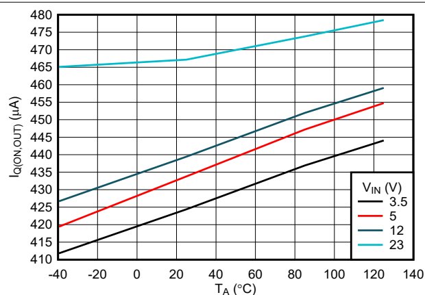
図 7-5. OUT Quiescent Current vs Temperature
