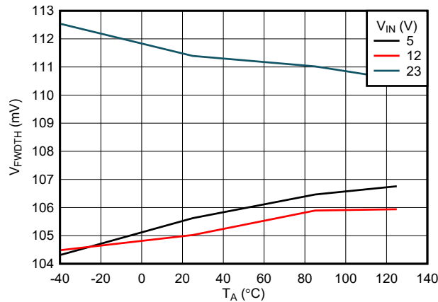
図 7-19. RCB - Forward Comparator Threshold vs Temperature
