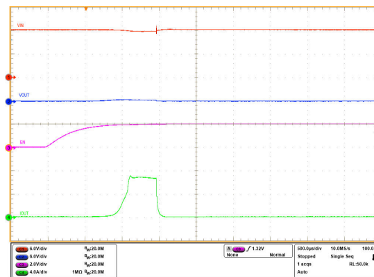
Figure 7-38. Power Up Into Short-Circuit
