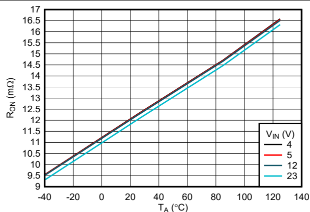
図 7-1. ON-Resistance vs Temperature
