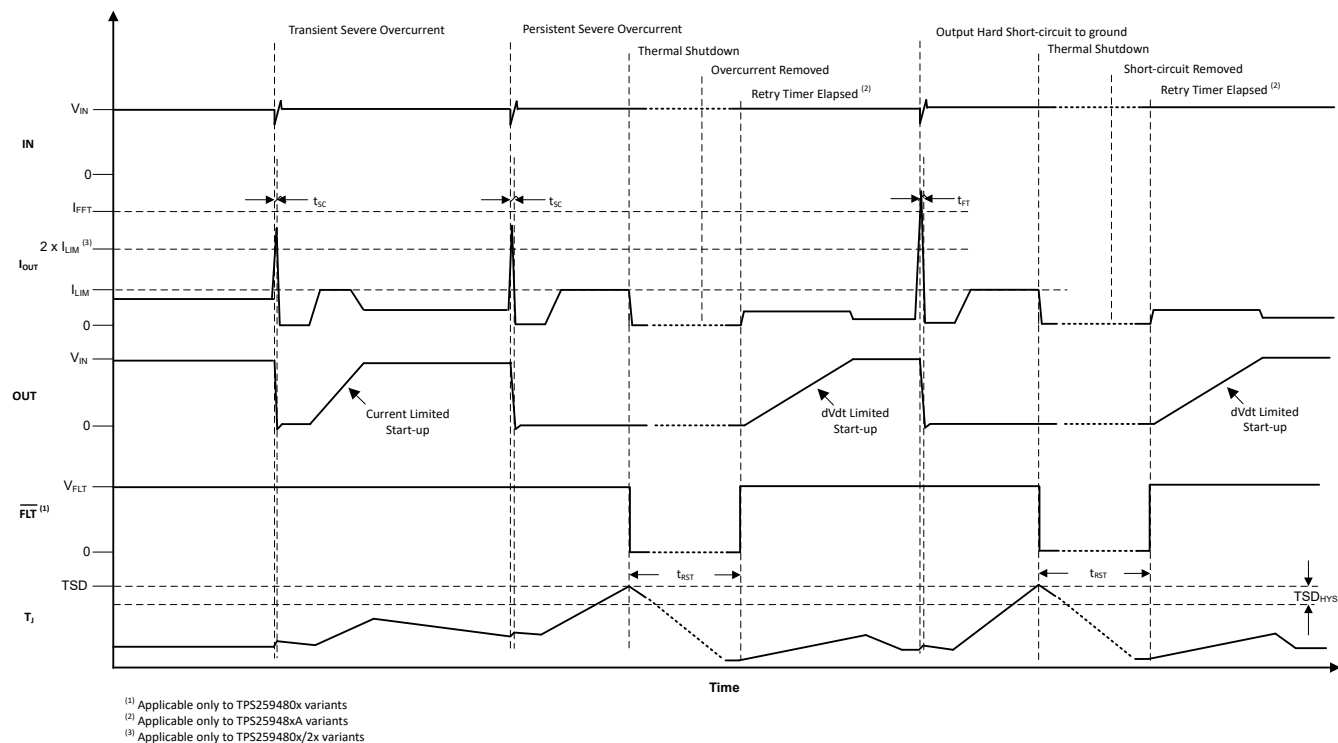
8-8. TPS259480x/2x Short-Circuit Response
