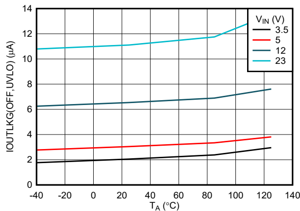
図 7-21. Reverse Leakage Current During OFF-State
