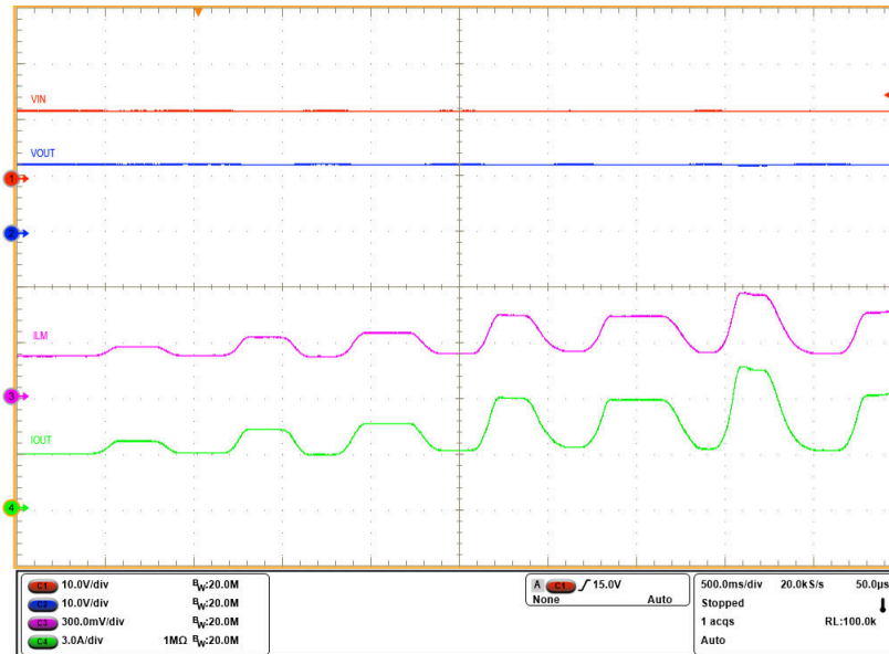
図 8-10. Analog Load Current Monitor Response
