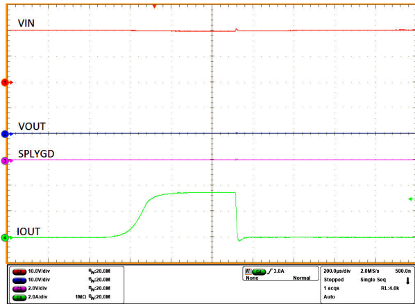
図 9-9. Wake up into Short Protection
