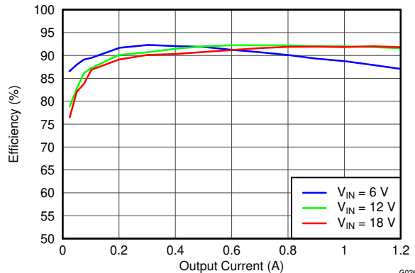
8-12. Efficiency vs Output Current
