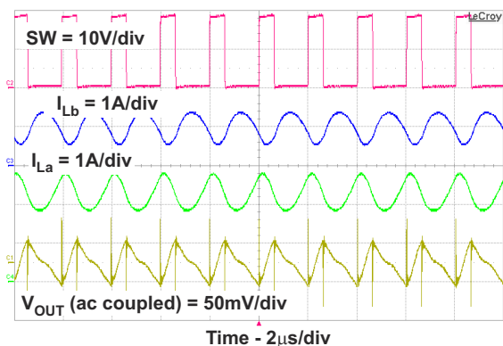
8-14. CCM PWM Operation
