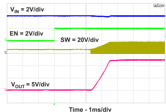
8-15. Output Voltage Soft-start
