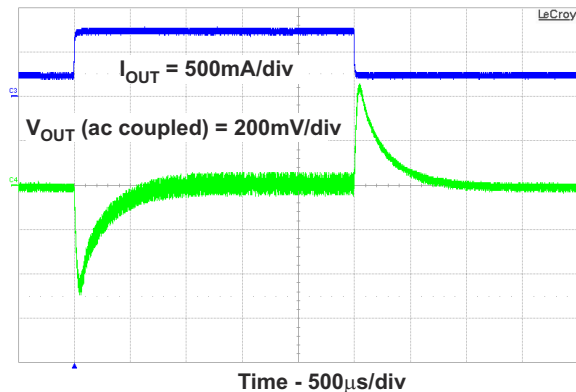
8-13. Load Transient Response
