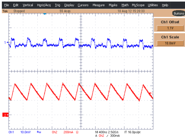
✎ 65. DCDCx Voltage Ripple and Inductor Current at 300 mA Load, 1.1-V V_{OUT}
