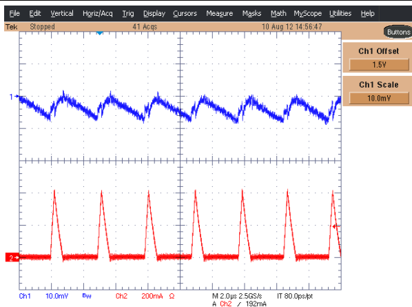
✎ 67. DCDCx Voltage Ripple and Inductor Current at 50 mA Load, 1.5-V V_{OUT}
