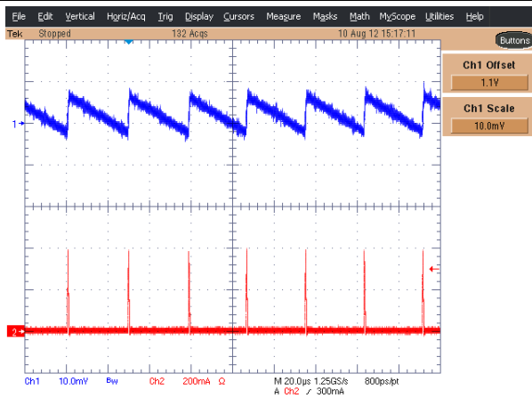
✎ 63. DCDCx Voltage Ripple and Inductor Current at 5 mA Load, 1.1-V V_{OUT}
