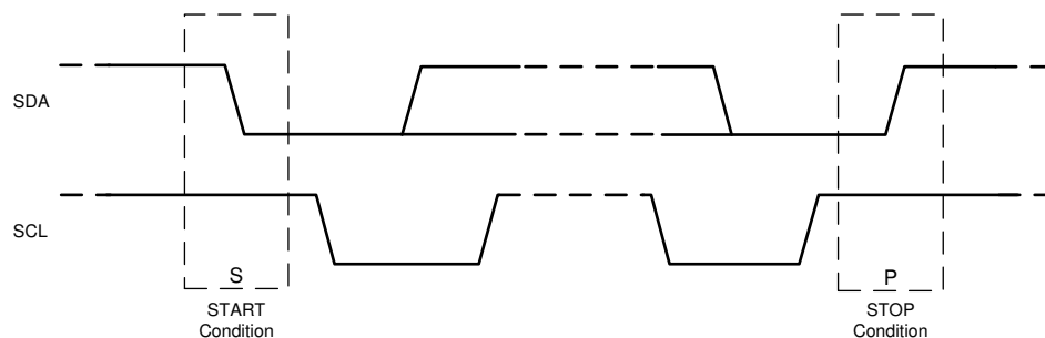
FIG 7-5. Start and Stop Sequences
