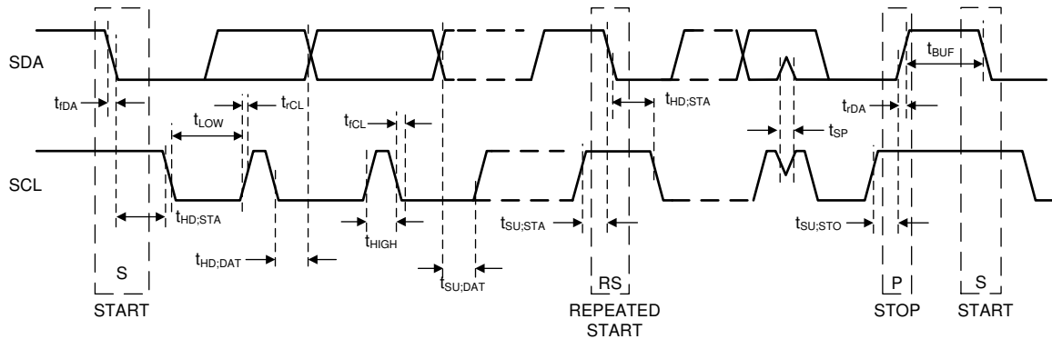
7-6. I 2 C-Compatible Timing
