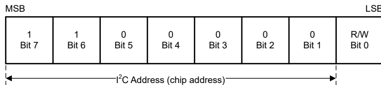
7-7. Example Device Address
