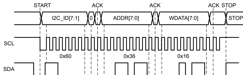
7-8. I 2 C Write Cycle without CRC
