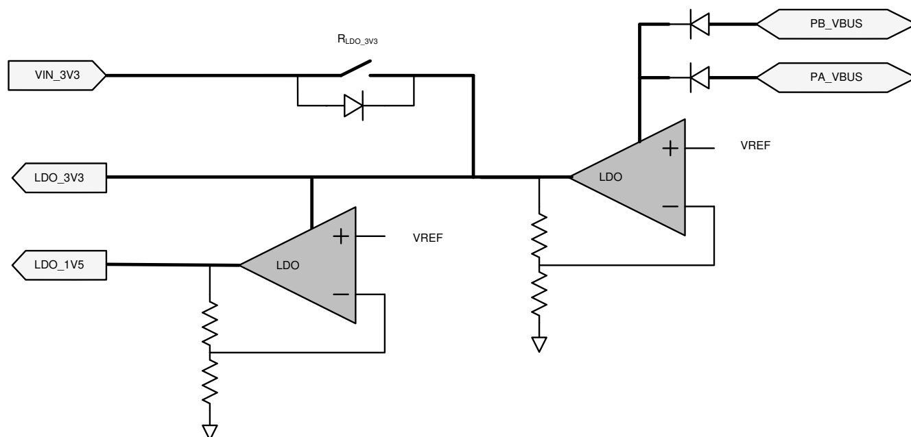
8-9. Power Supplies
