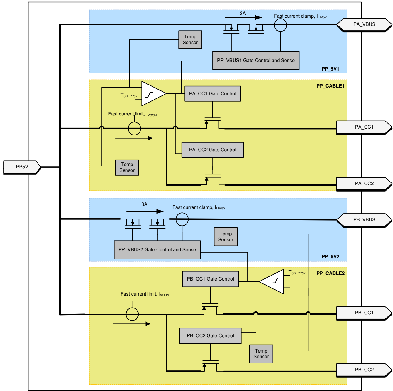
FIG 8-10. Port Power Switches
