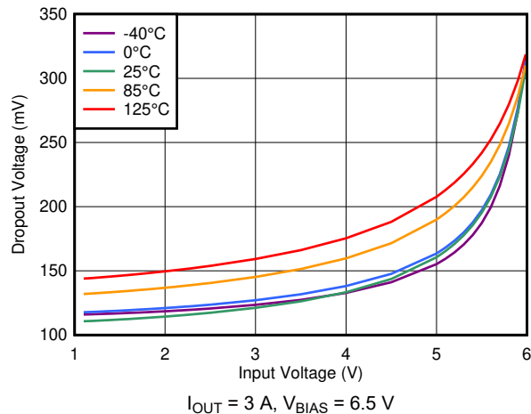
FIG 6-21. Dropout Voltage vs Input Voltage With Bias
