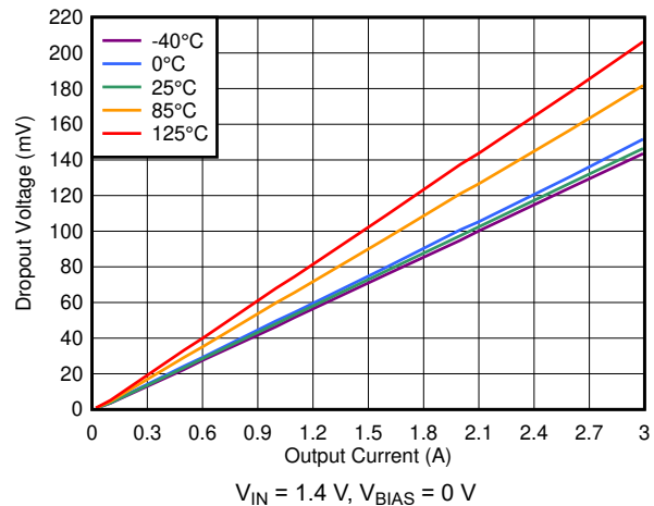
FIG 6-22. Dropout Voltage vs Output Current Without Bias
