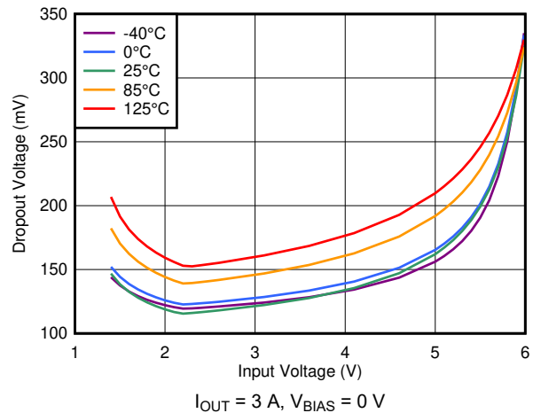
FIG 6-20. Dropout Voltage vs Input Voltage Without Bias
