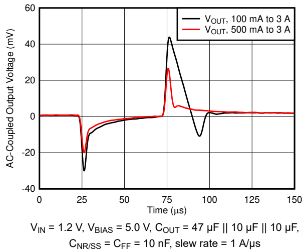
FIG 6-19. Load Transient vs Time and DC Load ( V_{OUT} = 0.9\text{ V} )
