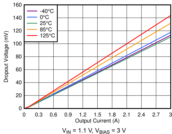
FIG 6-23. Dropout Voltage vs Output Current With Bias
