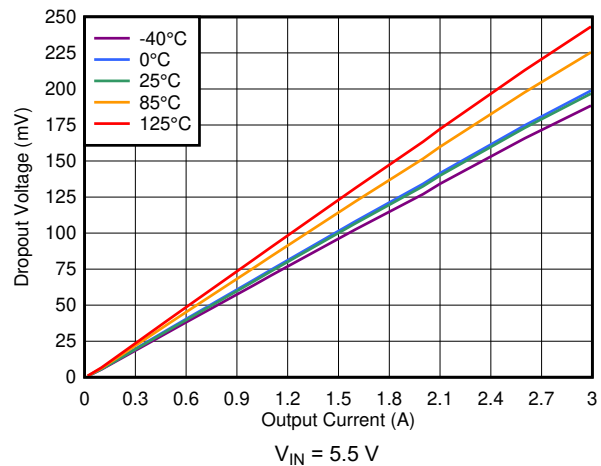
FIG 6-24. Dropout Voltage vs Output Current (High V_{IN} )
