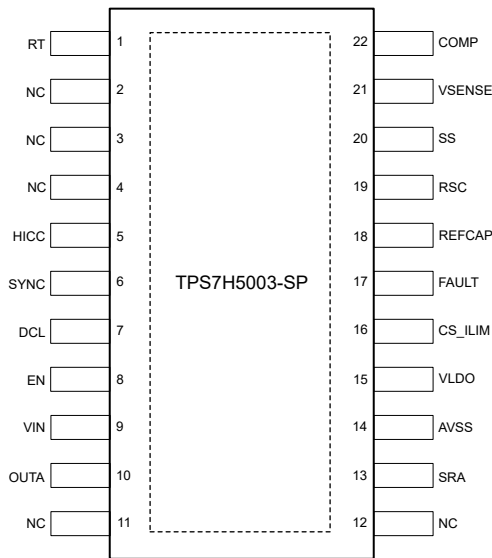
7-3. TPS7H5003-SP HFT Package 22-Pin CFP With Thermal Pad (Top View)
