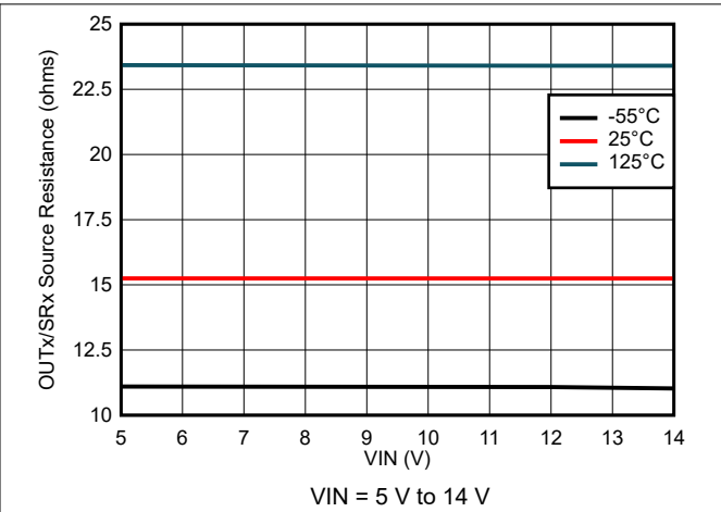
8-62. Output Source Resistance Variation
