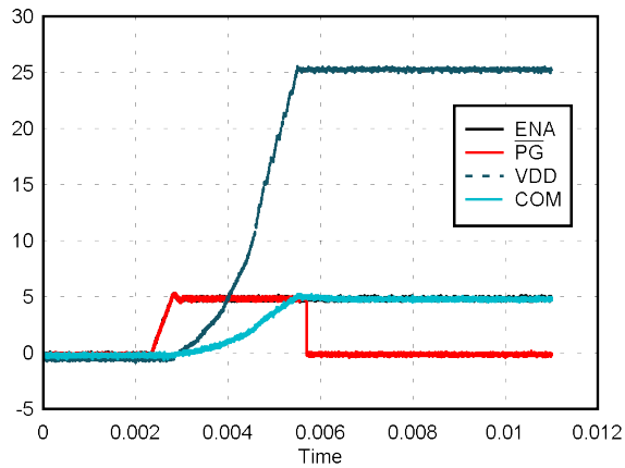
FIG 10-6. Start-up: V_{IN} = 24\text{ V} , V_{VDD-VEE} = 25\text{ V} , V_{COM-VEE} = 5\text{ V} , No Load
