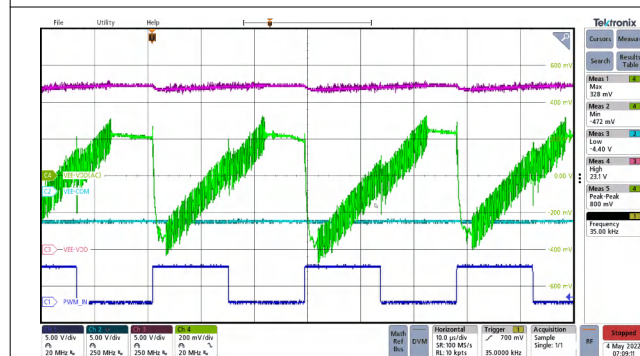
图 12-15. Ripple voltage: VDD-VEE Switching 100-nF Load at 35 kHz.
