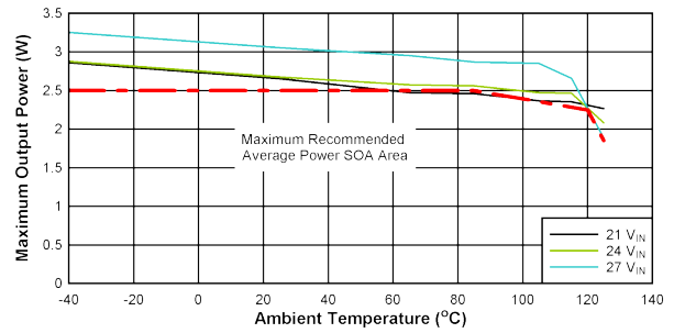
FIG 10-4. SOA Derating Curves: V_{\text{DD-VEE}} = 25 \text{ V} , V_{\text{COM-VEE}} = 5 \text{ V} , T_{\text{shut}} = 160^{\circ}\text{C} , No Load on V_{\text{COM-VEE}} .
