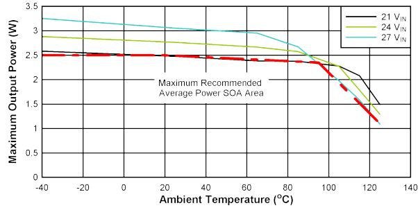
FIG 10-1. SOA Derating Curves: V_{\text{DD-VEE}} = 15 \text{ V} , V_{\text{COM-VEE}} = 5 \text{ V} , T_{\text{shut}} = 160^{\circ}\text{C} , No Load on V_{\text{COM-VEE}} .
