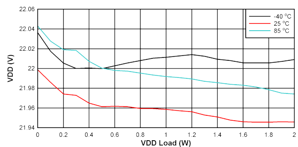
FIG 10-11. V_{VDD-VEE} Load Regulation: V_{IN} = 24\text{ V} , V_{VDD-VEE} = 22\text{ V} , V_{COM-VEE} = 4\text{ V}
