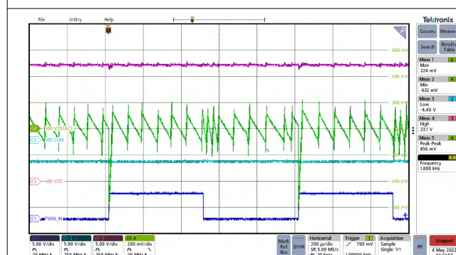
图 12-13. Ripple voltage: VDD-VEE Switching 100-nF Load at 1 kHz.
