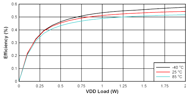
FIG 10-18. Efficiency vs Load on V_{DD-VEE} : V_{IN} = 27\text{ V} , V_{DD-VEE} = 22\text{ V} , V_{COM-VEE} = 4\text{ V} , No Load on V_{COM-VEE}
