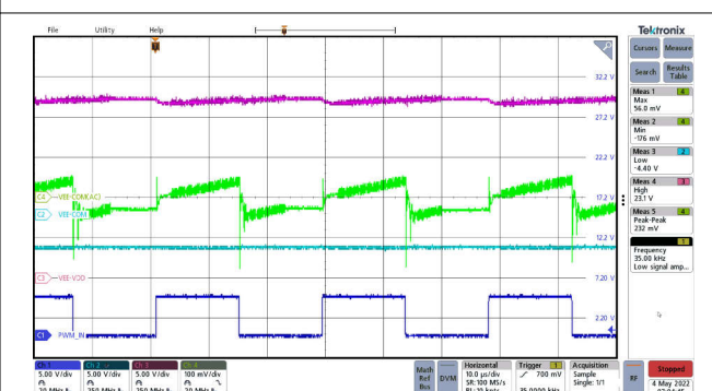
图 12-14. Ripple voltage: VEE-COM Switching 100-nF Load at 35 kHz.
