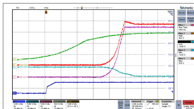
图 12-11. Power-Up Sequence.
