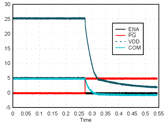
FIG 10-7. Shutdown: V_{IN} = 24\text{ V} , V_{VDD-VEE} = 25\text{ V} , V_{COM-VEE} = 5\text{ V} , No Load
