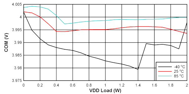
FIG 10-15. V_{COM-VEE} Load Regulation: V_{IN} = 27\text{ V} , V_{DD-VEE} = 22\text{ V} , V_{COM-VEE} = 4\text{ V}
