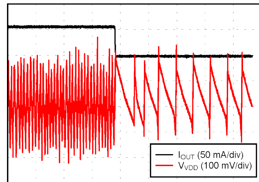
FIG 10-9. Load Transient Response: 1 W to No Load, V_{IN} = 24\text{ V} , V_{VDD-VEE} = 25\text{ V} , V_{COM-VEE} = 5\text{ V}
