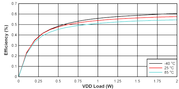
FIG 10-17. Efficiency vs Load on V_{DD-VEE} : V_{IN} = 24\text{ V} , V_{DD-VEE} = 22\text{ V} , V_{COM-VEE} = 4\text{ V} , No Load on V_{COM-VEE}
