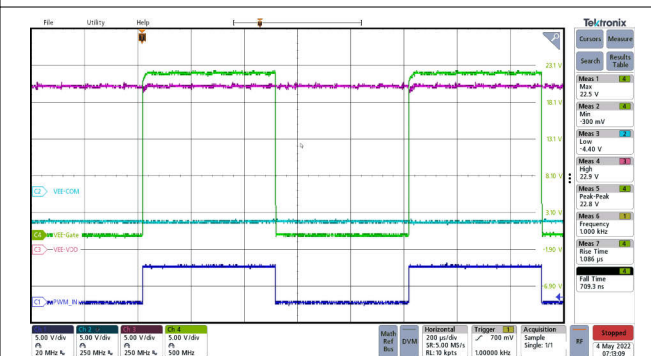
图 12-16. Gate Waveform Switching 100 nF at 1 kHz.
