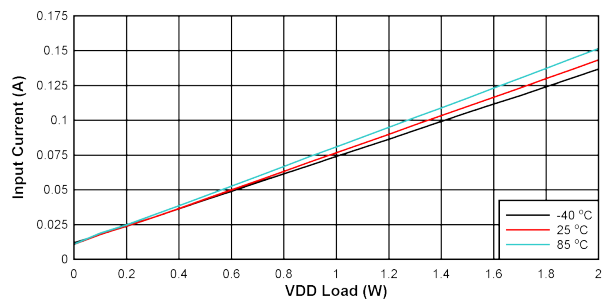
FIG 10-20. Input Current vs Load on V_{DD-VEE} : V_{IN} = 24\text{ V} , V_{DD-VEE} = 22\text{ V} , V_{COM-VEE} = 4\text{ V} , No Load on V_{COM-VEE}
