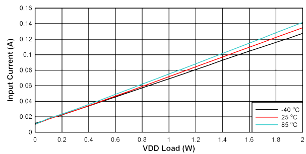
FIG 10-21. Input Current vs Load on V_{DD-VEE} : V_{IN} = 27\text{ V} , V_{DD-VEE} = 22\text{ V} , V_{COM-VEE} = 4\text{ V} , No Load on V_{COM-VEE}
