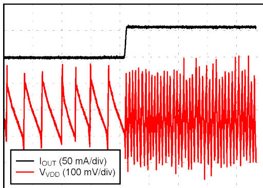
FIG 10-8. Load Transient Response: No Load to 1 W, V_{IN} = 24\text{ V} , V_{VDD-VEE} = 25\text{ V} , V_{COM-VEE} = 5\text{ V}
