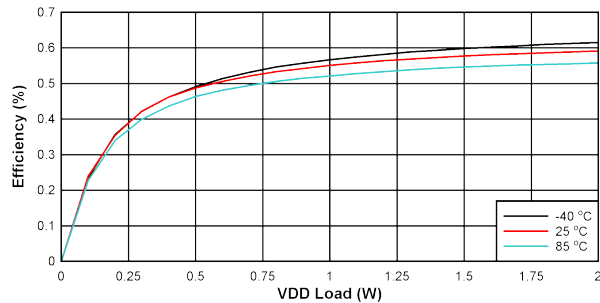
FIG 10-16. Efficiency vs Load on V_{DD-VEE} : V_{IN} = 21\text{ V} , V_{DD-VEE} = 22\text{ V} , V_{COM-VEE} = 4\text{ V} , No Load on V_{COM-VEE}
