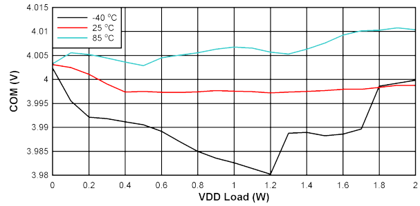
FIG 10-13. V_{COM-VEE} Load Regulation: V_{IN} = 21\text{ V} , V_{DD-VEE} = 22\text{ V} , V_{COM-VEE} = 4\text{ V}
