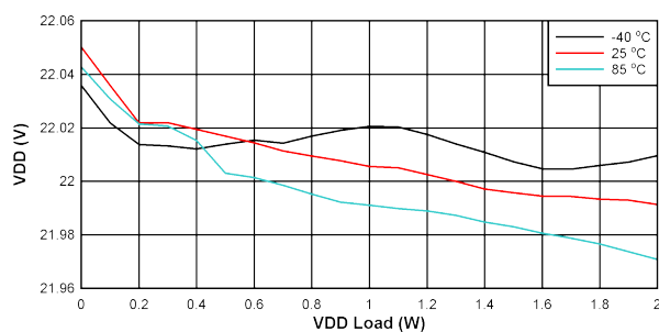
FIG 10-10. V_{VDD-VEE} Load Regulation: V_{IN} = 21\text{ V} , V_{VDD-VEE} = 22\text{ V} , V_{COM-VEE} = 4\text{ V}
