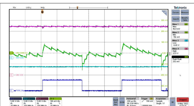
图 12-12. Ripple voltage: VEE-COM Switching 100-nF Load at 1 kHz.
