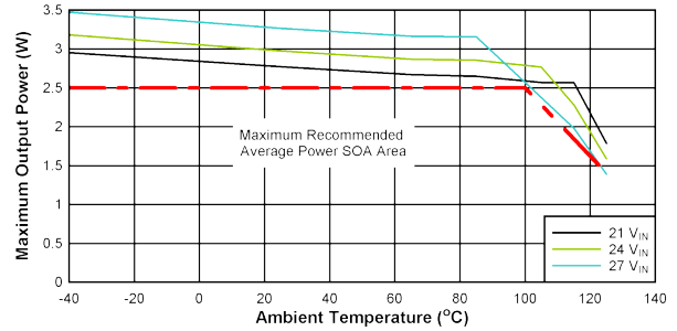
FIG 10-2. SOA Derating Curves: V_{\text{DD-VEE}} = 18 \text{ V} , V_{\text{COM-VEE}} = 5 \text{ V} , T_{\text{shut}} = 160^{\circ}\text{C} , No Load on V_{\text{COM-VEE}} .
