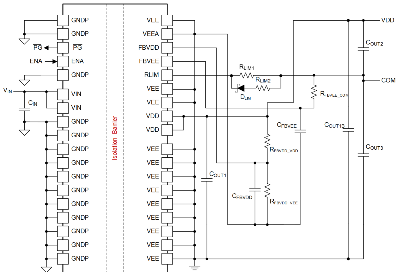
FIG 12-9. Dual output application schematic configured for V_{COM\_VEE} regulation = 2.5V
