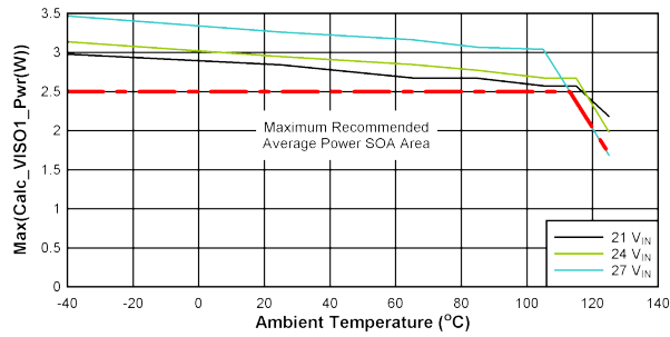
FIG 10-3. SOA Derating Curves: V_{\text{DD-VEE}} = 22 \text{ V} , V_{\text{COM-VEE}} = 4 \text{ V} , T_{\text{shut}} = 160^{\circ}\text{C} , No Load on V_{\text{COM-VEE}} .
