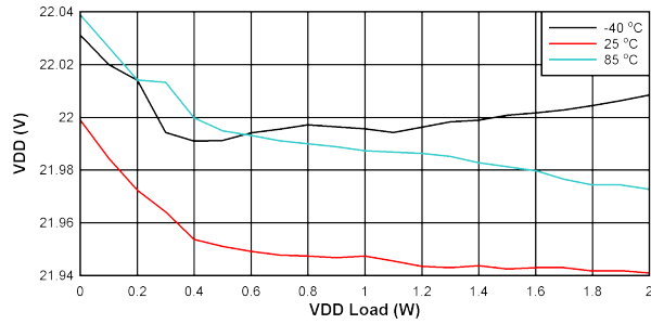
FIG 10-12. V_{DD-VEE} Load Regulation: V_{IN} = 27\text{ V} , V_{DD-VEE} = 22\text{ V} , V_{COM-VEE} = 4\text{ V}
