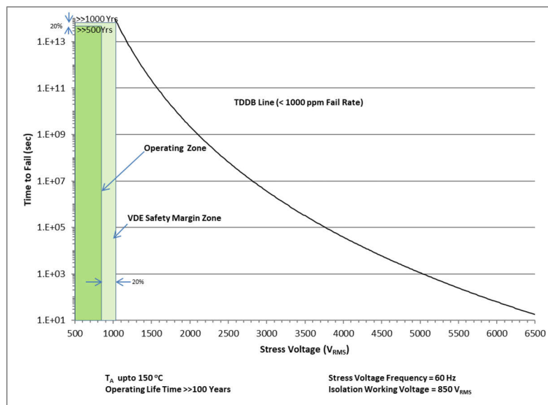
FIG 9-1. TDDB: Insulation Lifetime Projection for 850 Vrms Working Voltage.
