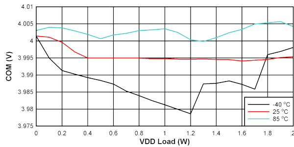
FIG 10-14. V_{COM-VEE} Load Regulation: V_{IN} = 24\text{ V} , V_{DD-VEE} = 22\text{ V} , V_{COM-VEE} = 4\text{ V}
