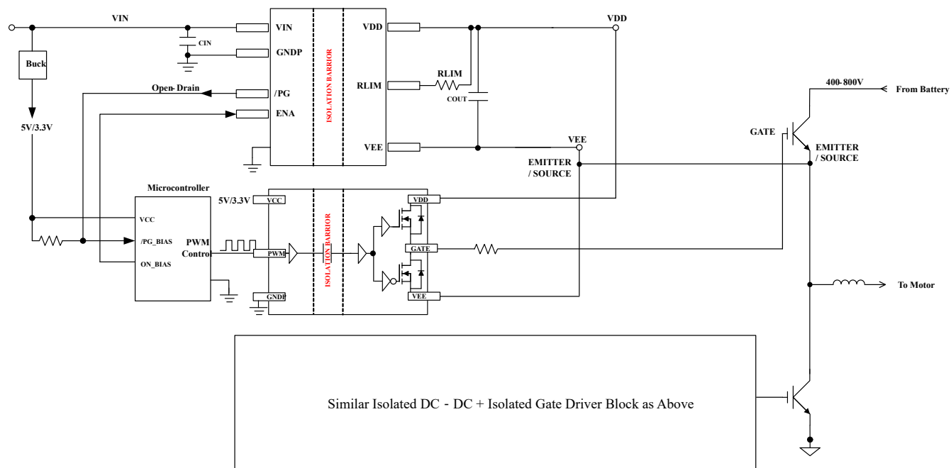
图 12-19. Single Output System Configuration
