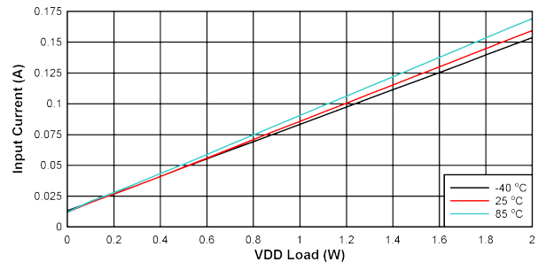
FIG 10-19. Input Current vs Load on V_{DD-VEE} : V_{IN} = 21\text{ V} , V_{DD-VEE} = 22\text{ V} , V_{COM-VEE} = 4\text{ V} , No Load on V_{COM-VEE}
