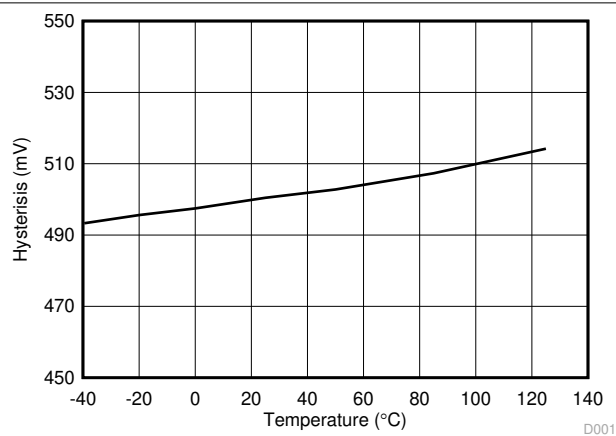
FIG 7-19. VDD 8-V UVLO Hysteresis vs Temperature
