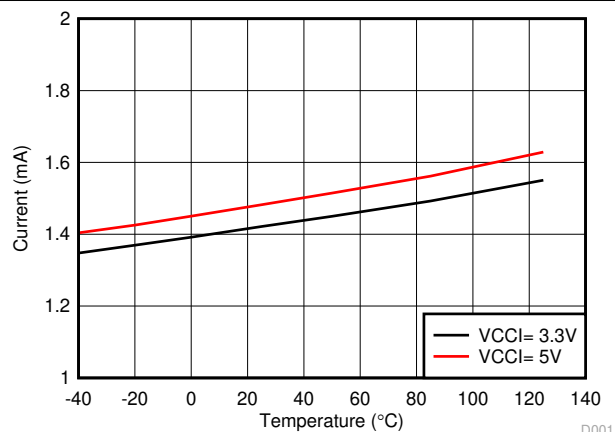
7-9. I_{VCCI} Quiescent Supply Current vs Temperature (No Load, Input Low, No Switching)
