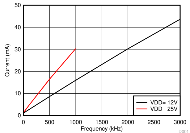
7-5. Per Channel Current Consumption ( I_{VDDA/B} ) vs Frequency (1-nF Load, VDD = 12 V or 25 V)
