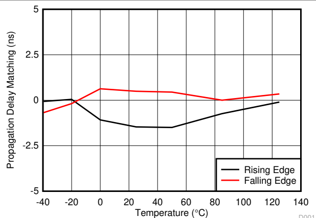
FIG 7-16. Propagation Delay Matching ( t_{DM} ) vs Temperature
