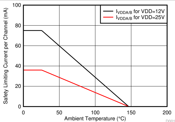
7-2. Thermal Derating Curve for Safety-Related Limiting Current (Current in Each Channel with Both Channels Running Simultaneously)
