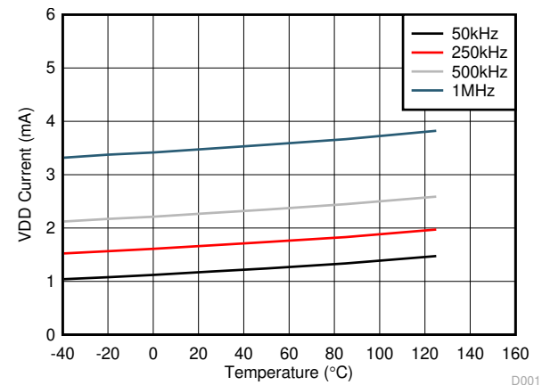
7-7. Per Channel ( I_{VDDA/B} ) Supply Current Vs. Temperature (No Load, Different Switching Frequencies)
