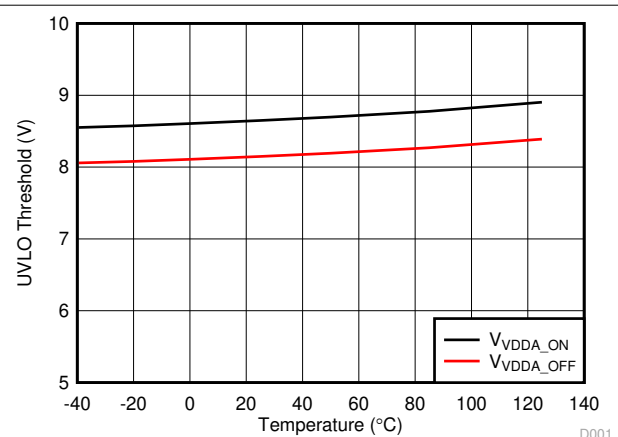
FIG 7-20. VDD 8-V UVLO Threshold vs Temperature
