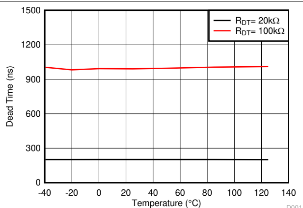
Figure 7-24. Dead Time vs Temperature (with R_{DT} = 20\text{ k}\Omega and 100\text{ k}\Omega )
