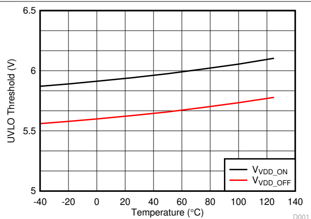
FIG 7-18. VDD 5-V UVLO Threshold vs Temperature
