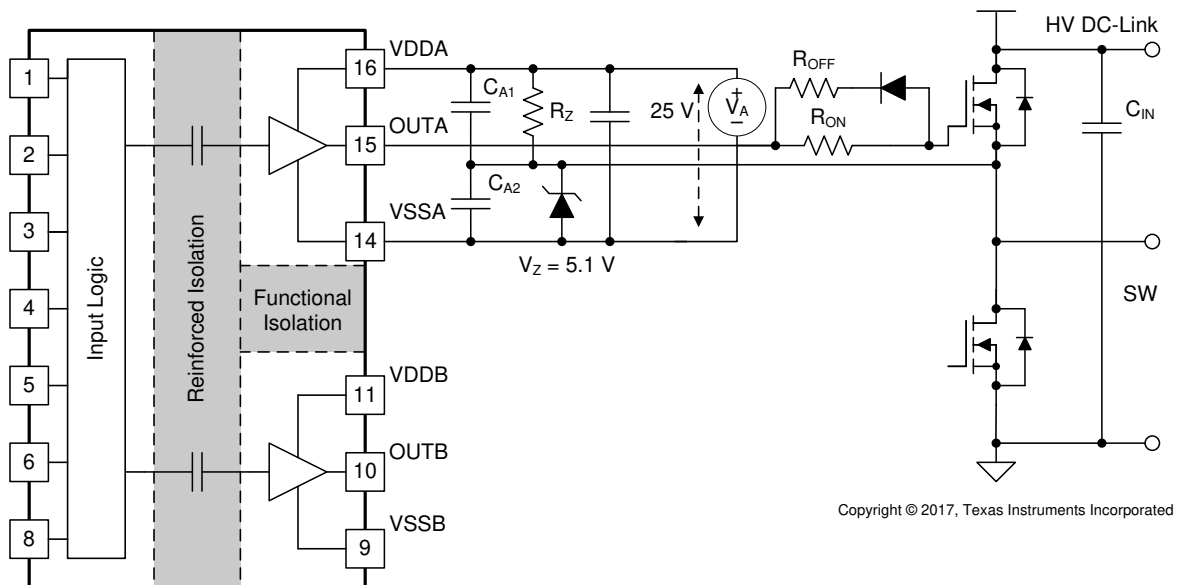
☒ 10-2. Negative Bias with Zener Diode on Iso-Bias Power Supply Output
