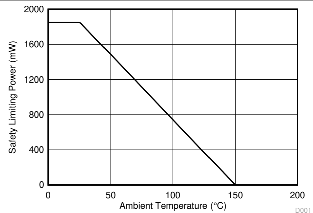
7-3. Thermal Derating Curve for Safety-Related Limiting Power
