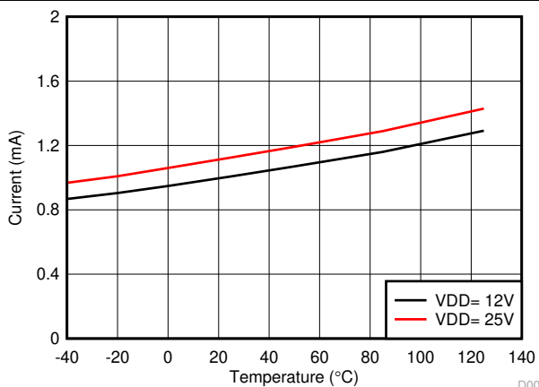
7-8. Per Channel ( I_{VDDA/B} ) Quiescent Supply Current vs Temperature (No Load, Input Low, No Switching)
