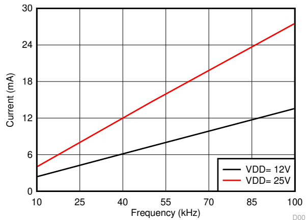
7-6. Per Channel Current Consumption ( I_{VDDA/B} ) vs Frequency (10-nF Load, VDD = 12 V or 25 V)
