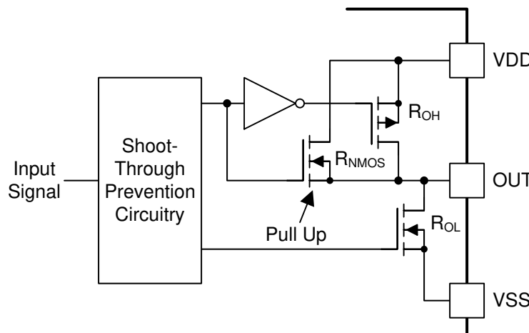
图 9-2. Output Stage
