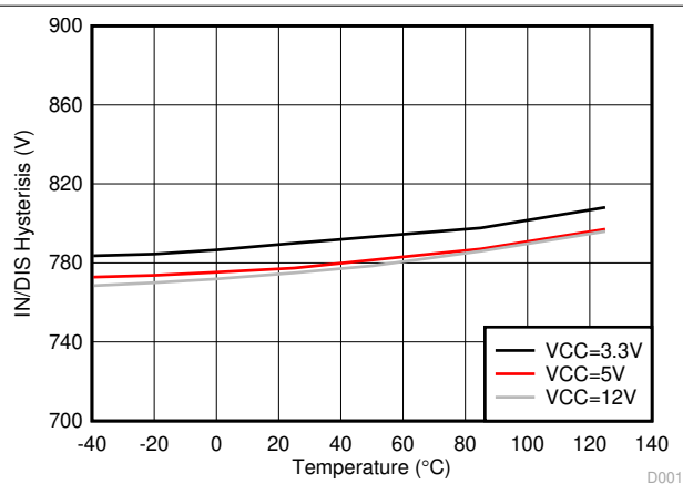
FIG 7-21. IN/DIS Hysteresis vs Temperature
