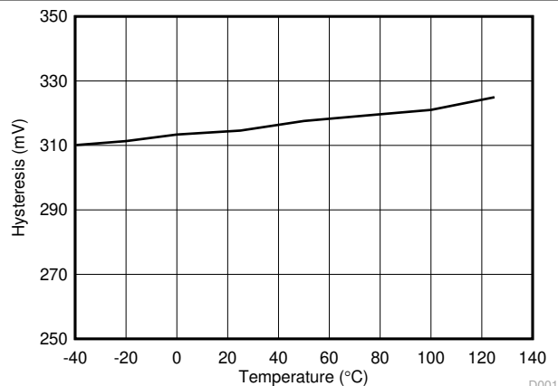
FIG 7-17. VDD 5-V UVLO Hysteresis vs Temperature
