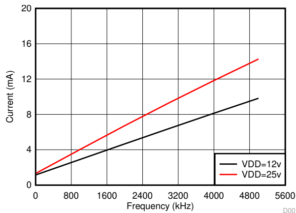
7-4. Per Channel Current Consumption vs Frequency (No Load, VDD = 12 V or 25 V)
