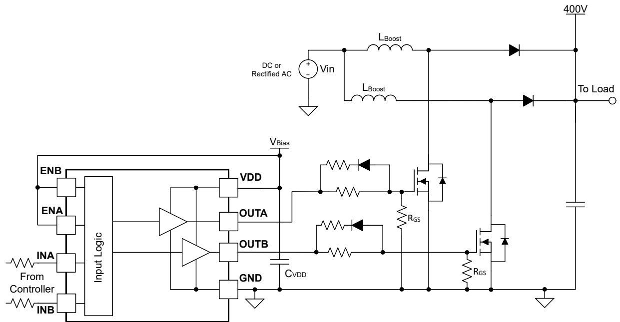
8-1. UCC27624-Q1 Typical Application Diagram
