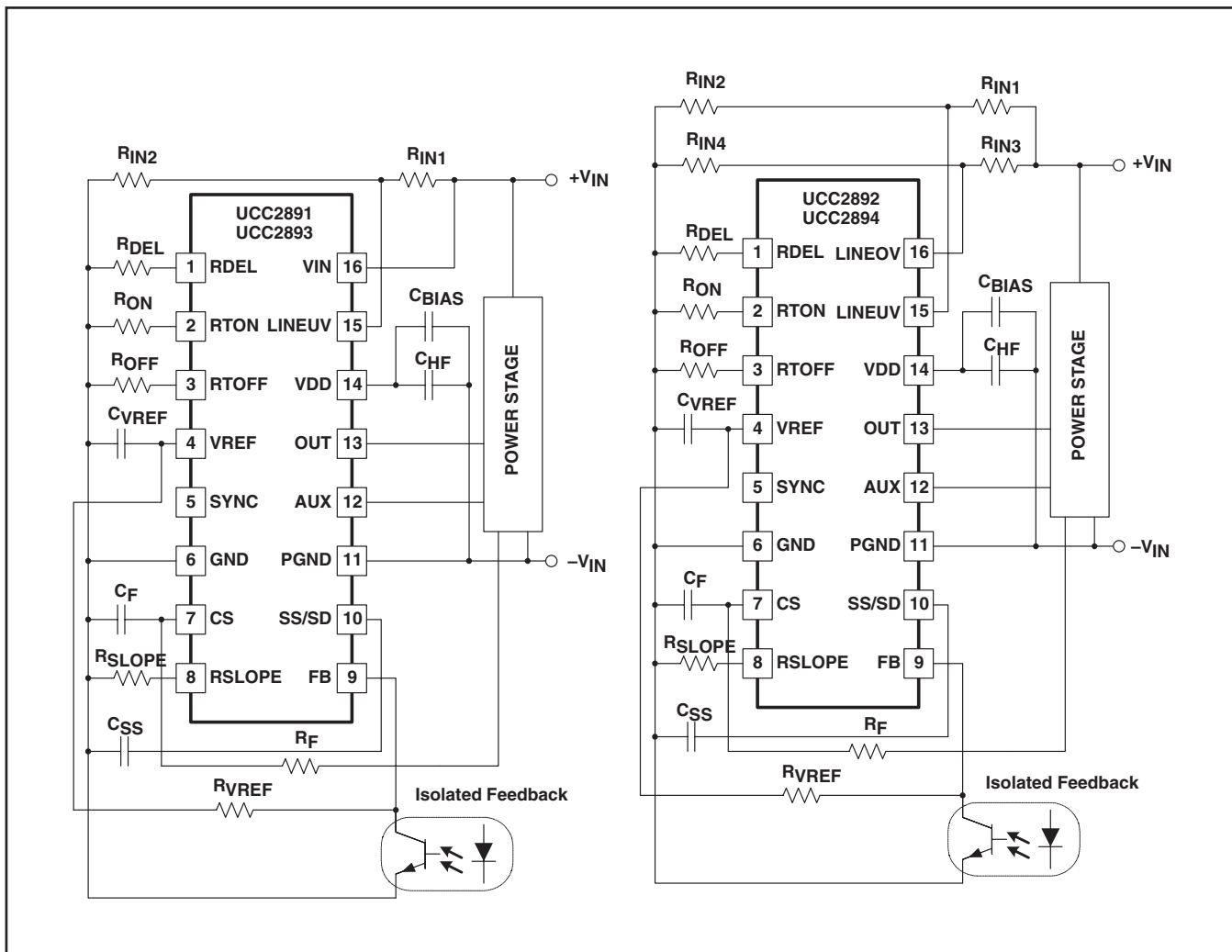
図 7. UCC289x Typical Setup
