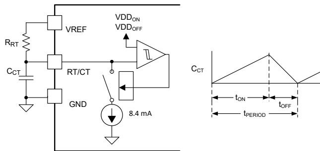
FIG 8-4. Oscillator Circuit
