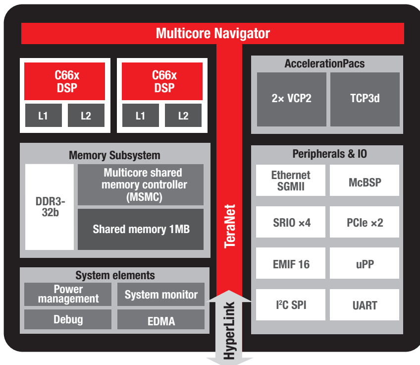
▲ Figure 1: TMS320C6657 block diagram
