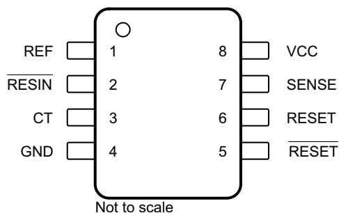
FIG 5-1. D or P Package 8-Pin SOIC or PDIP Top View
