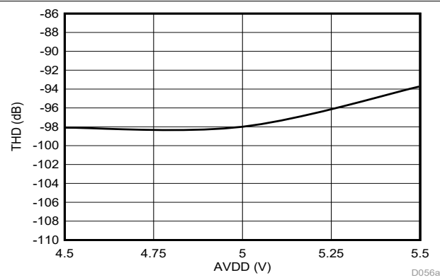
FIG 6-23. Total Harmonic Distortion vs High-Side Supply Voltage (5 V, nom)
