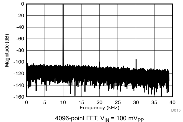
FIG 6-35. Frequency Spectrum With 10-kHz Input Signal
