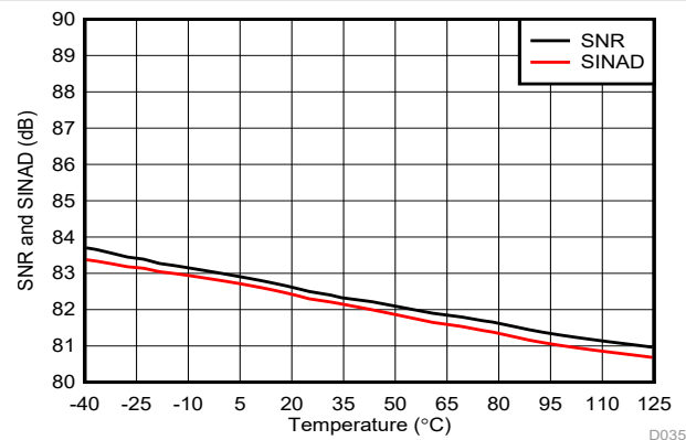
FIG 6-19. Signal-to-Noise Ratio and Signal-to-Noise + Distortion vs Temperature
