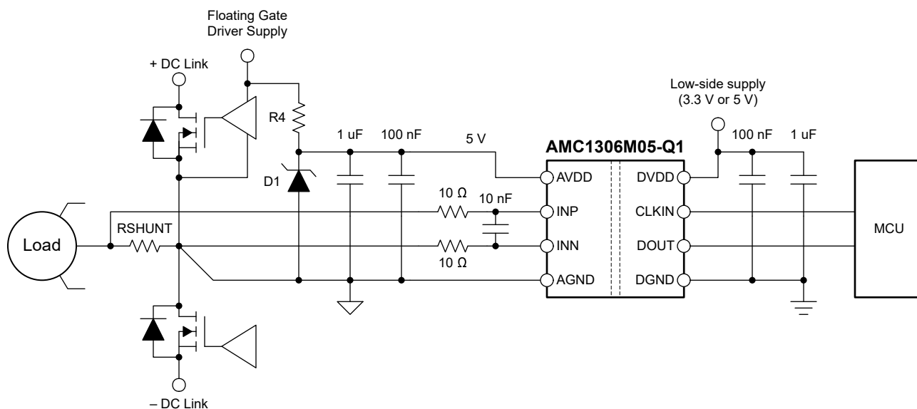
図 8-1. Using the AMC1306M05-Q1 for Current Sensing in a Typical Application
