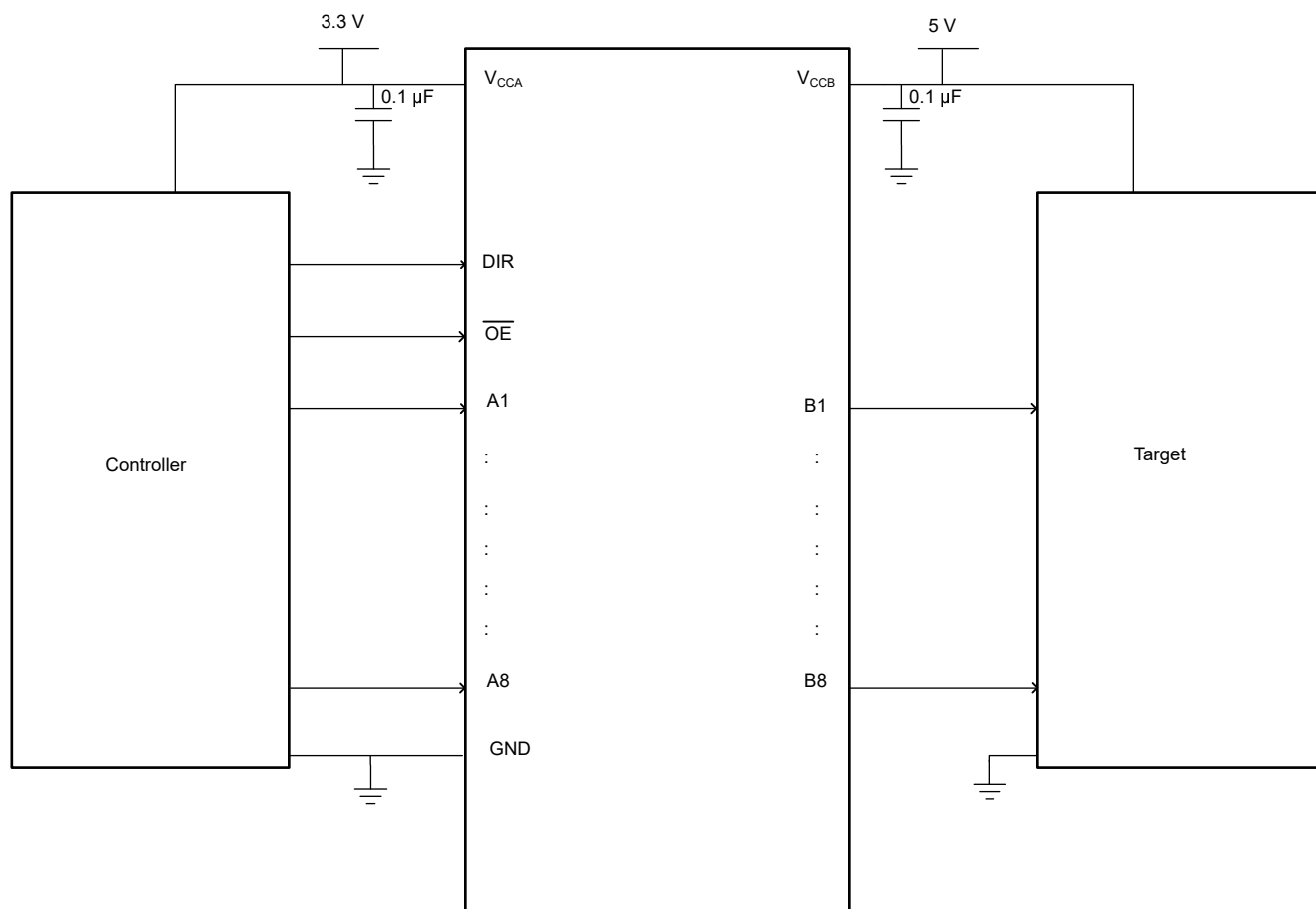
図 9-1. Typical Application
