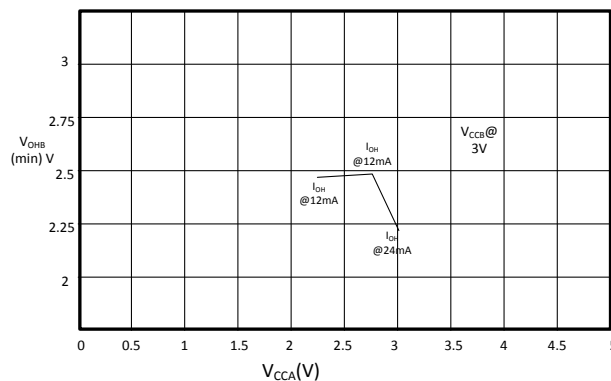
FIG 9-2. V_{OHB(min)} vs V_{CCA}
