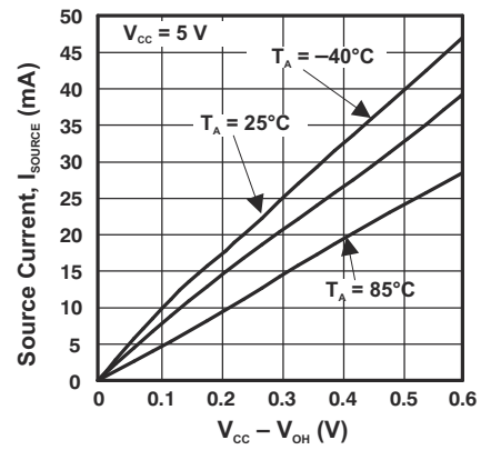
FIG 6-12. I/O Source Current vs Output High Voltage
