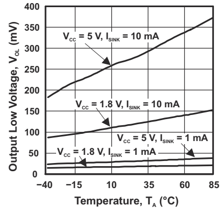
FIG 6-8. I/O Low Voltage vs Temperature
