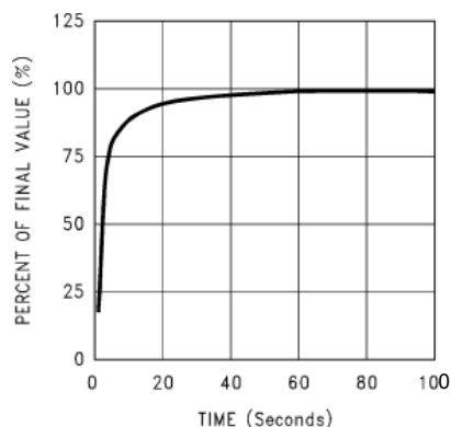
図 6-7. Thermal Response in Still Air Without a Heat Sink (Legacy chip)
