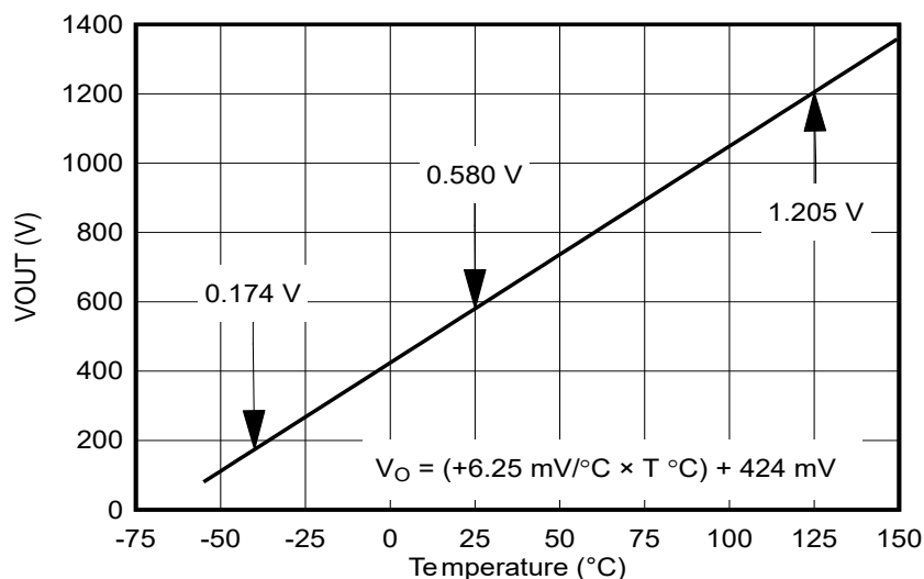
FIG 8-4. LM60 Output Transfer Function
