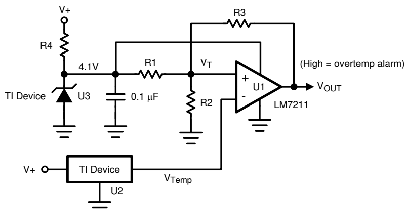
FIG 8-5. Centigrade Thermostat
