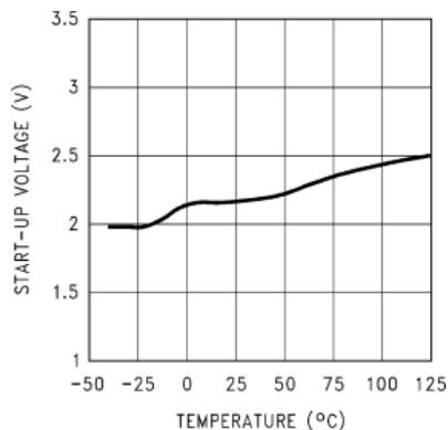
図 6-9. Start-Up Voltage vs Temperature (Legacy chip)
