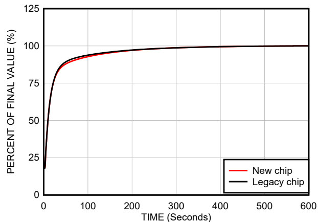
図 6-8. Thermal Response in Still Air Without a Heat Sink (Both Legacy and New chip in the new test setup)
