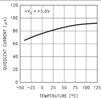
図 6-11. Quiescent Current vs Temperature (Legacy chip)
