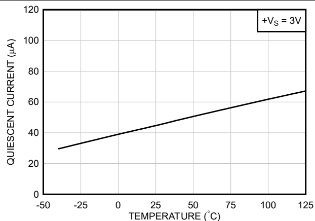
図 6-12. Quiescent Current vs Temperature (New chip)
