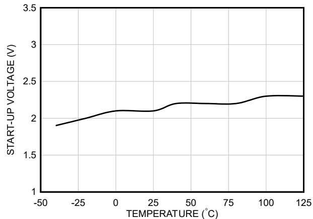
図 6-10. Start-Up Voltage vs Temperature (New chip)
