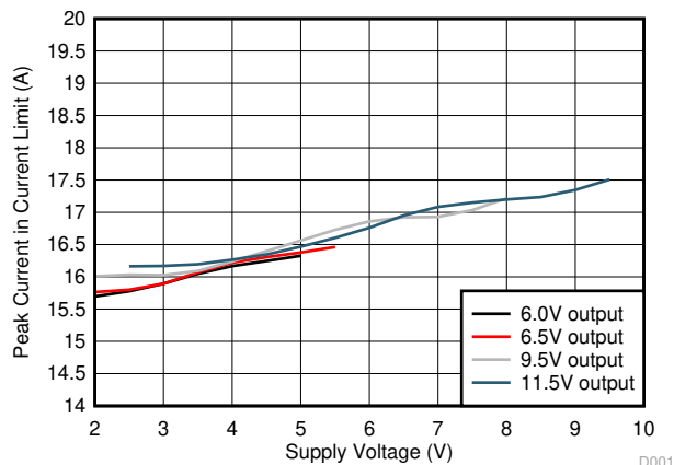
7-1. Peak Inductor Current vs Supply Voltage ( F_{SW} = 440 \text{ kHz} , R_S = 7 \text{ m}\Omega , R_F = 100 \text{ }\Omega , C_F = 2.2 \text{ nF} )
