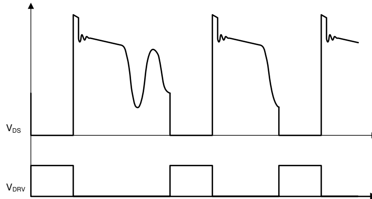
Figure 7-1. Valley-Skipping Mode
