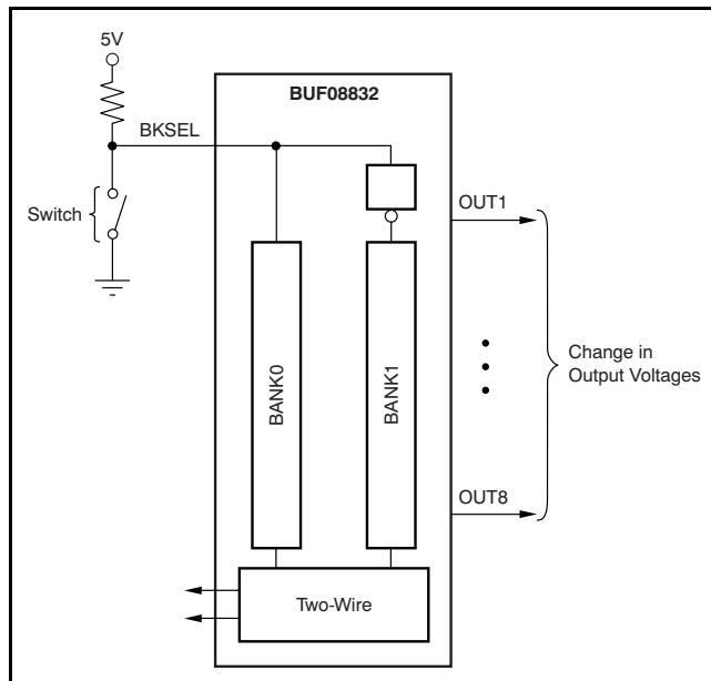
Figure 21. Gamma Control
