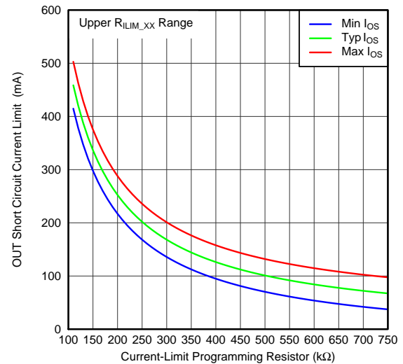
Figure 42. Current Limit Setting vs Programming Resistor
