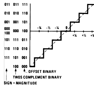
Figure 13. ADC Codes
