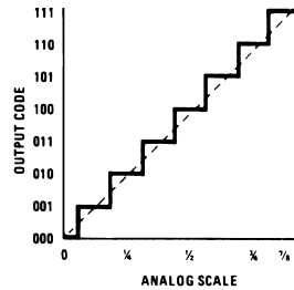
Figure 12. (a) Zero to + Full-Scale
