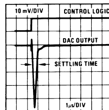
Figure 11. DAC Slew and Settling Time
