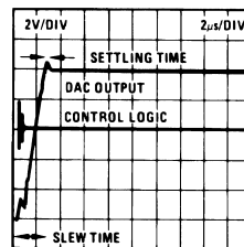
Figure 10. (a) Full-Scale Step
